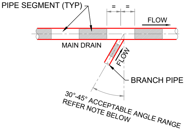
PREFERRED BRANCH LOCATION ALONG MAIN DRAIN PLAN
