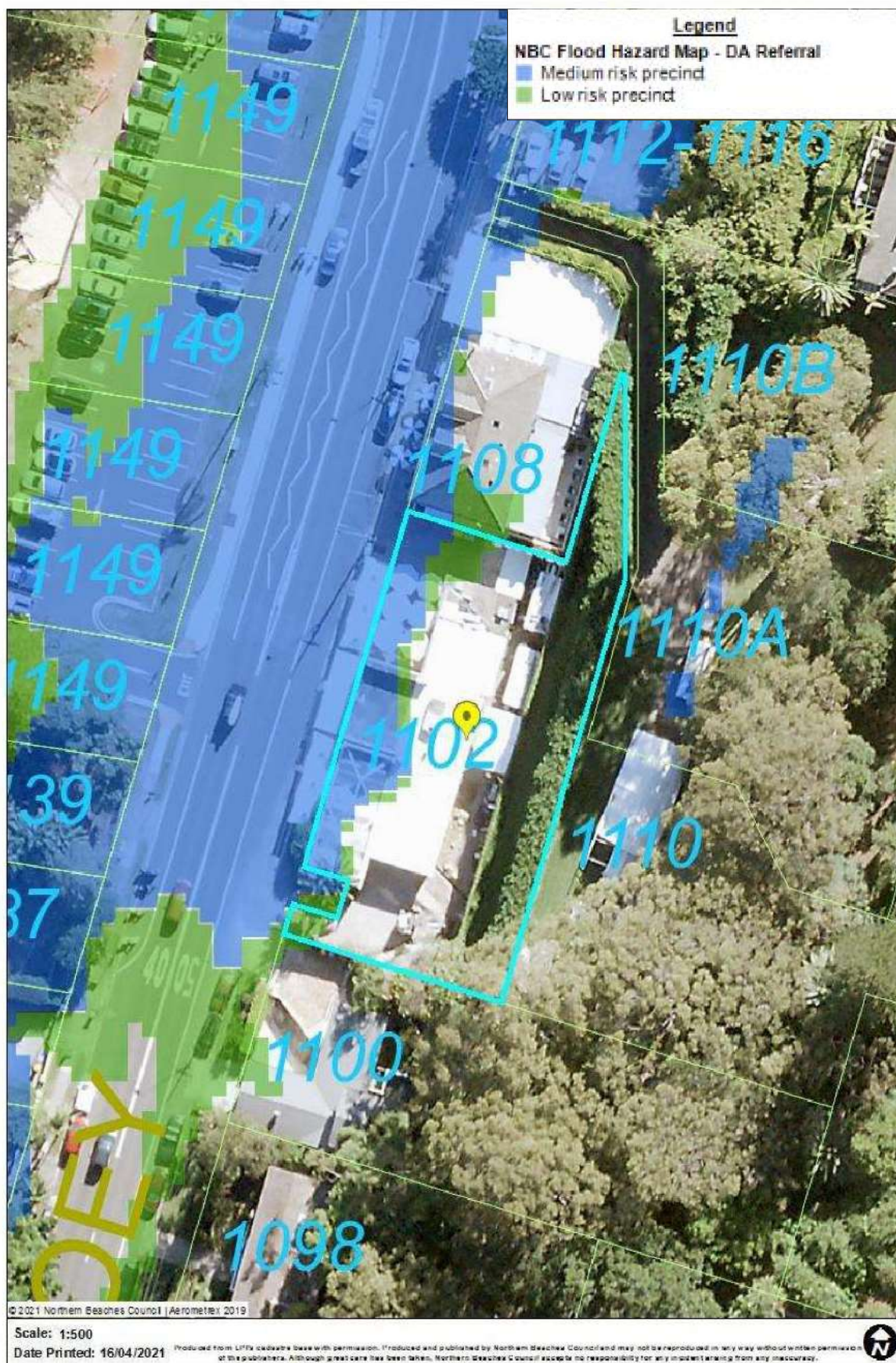
Figure 4.1 – Flood Risk Precinct Map (Northern Beaches Council, 2021)
