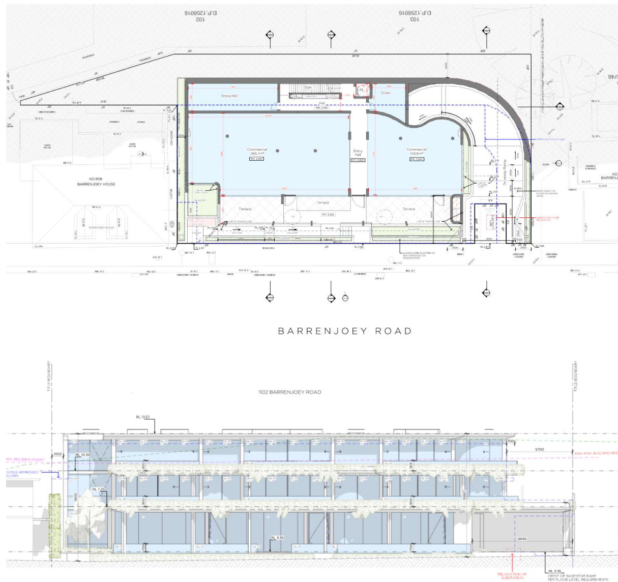
Figure 3.2 – Proposed Ground Floor Plan and West Elevation (Rob Mills Architects, 2021)
