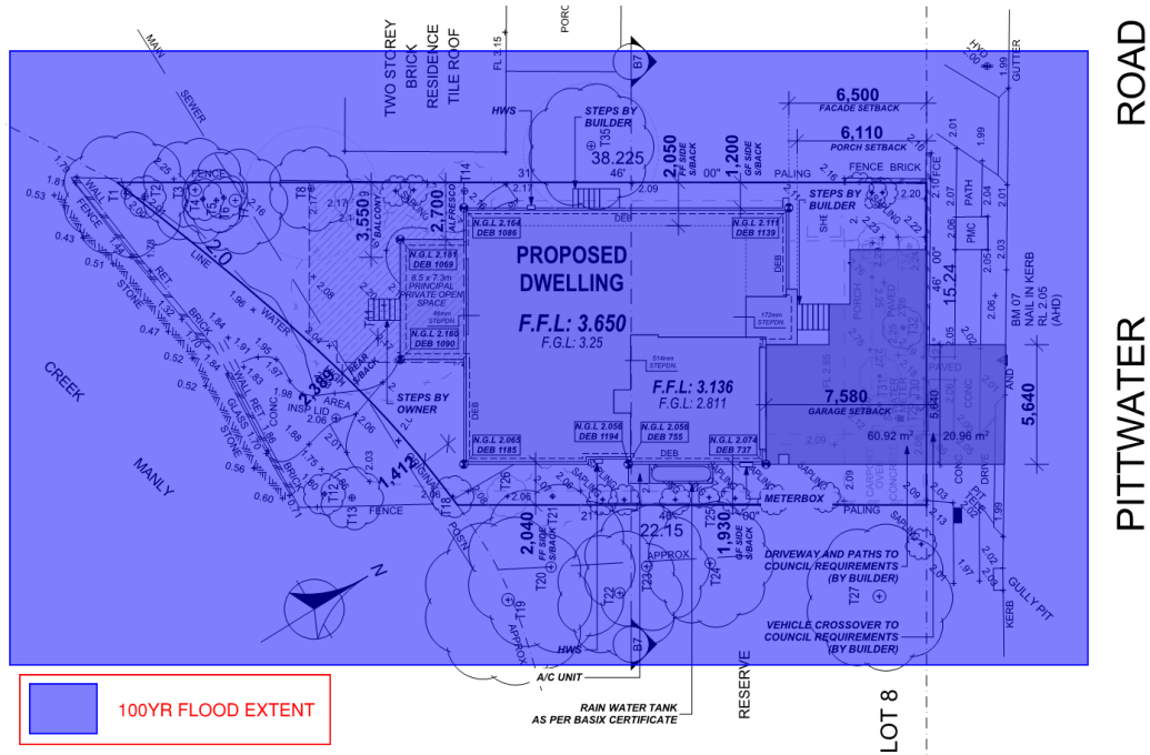
Figure 4 - 100YR Flood Extent (Source: Zait Engineering Solutions)
