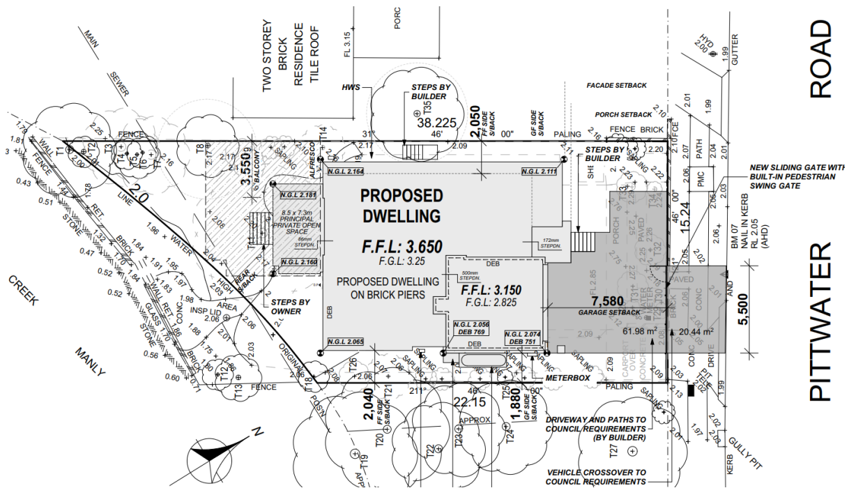
Figure 3 - Post-Developed Site Plan (Source: Hall & Hart dated 23/02/21)
