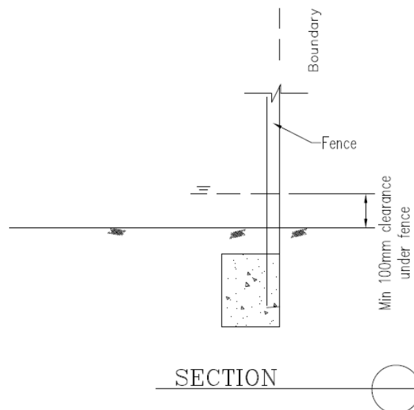
Figure 5 - Flood Fencing Detail
