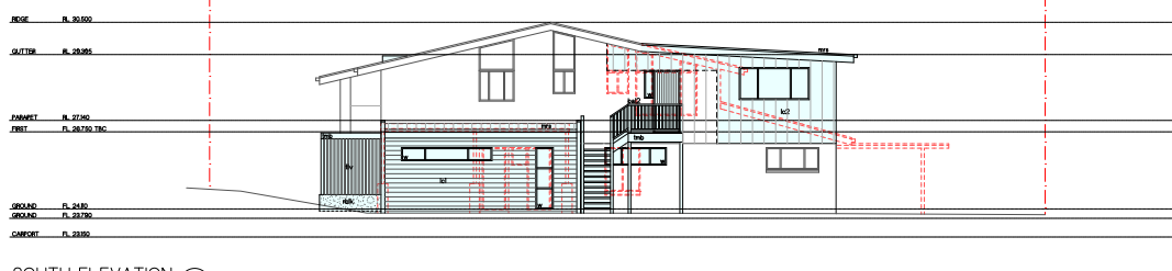
SOUTH ELEVATION Scale 1:100
