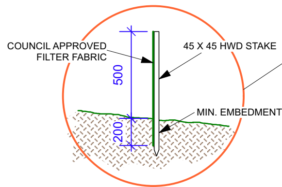
SEDIMENT CONTROL FENCE SECTION
