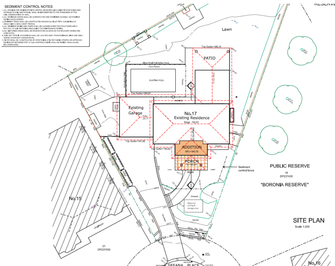
Figure 2: Roof/site plan.
