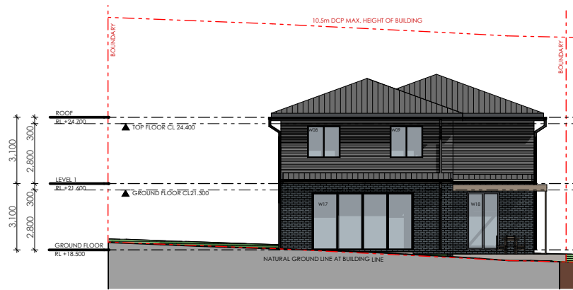
1 EAST ELEVATION 1:250
