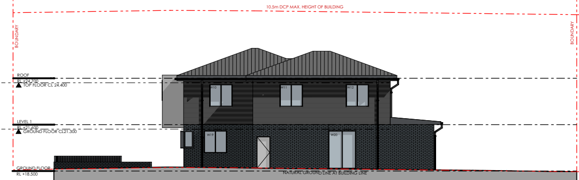
4 SOUTH ELEVATION 1:250
