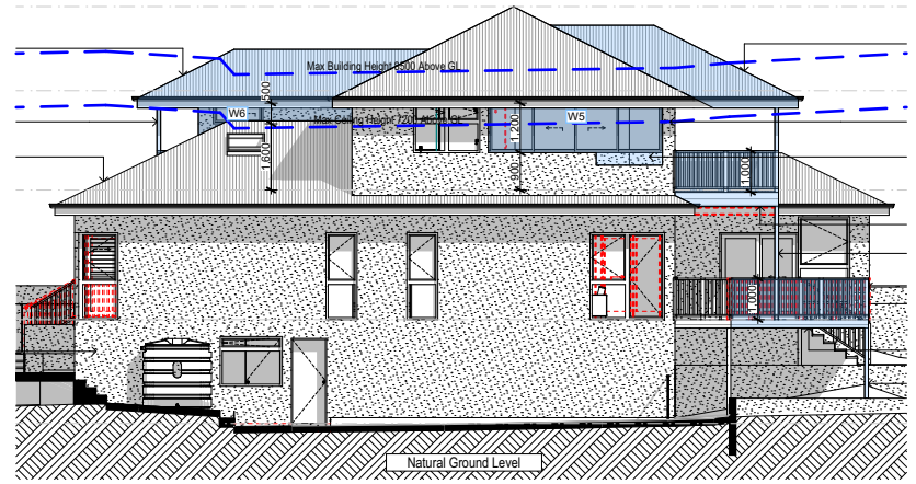
E-02 East 1:200
