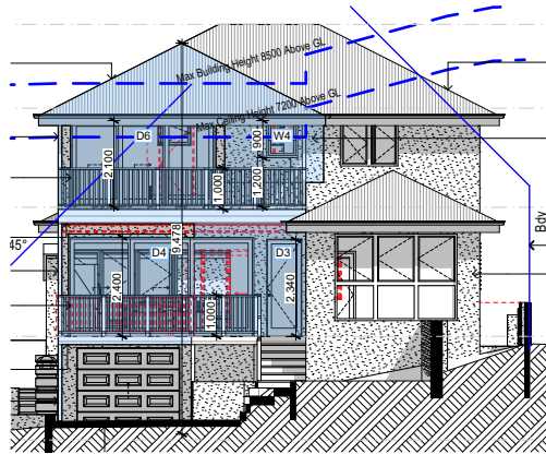
E-01 North 1:200
