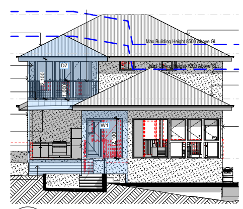
E-03 South 1:200
