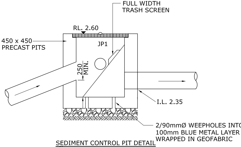
SEDIMENT CONTROL PIT DETAIL
