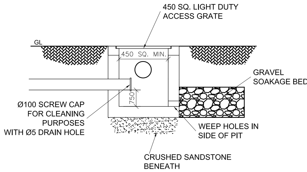
MAINTENANCE PIT DETAIL 1:100
