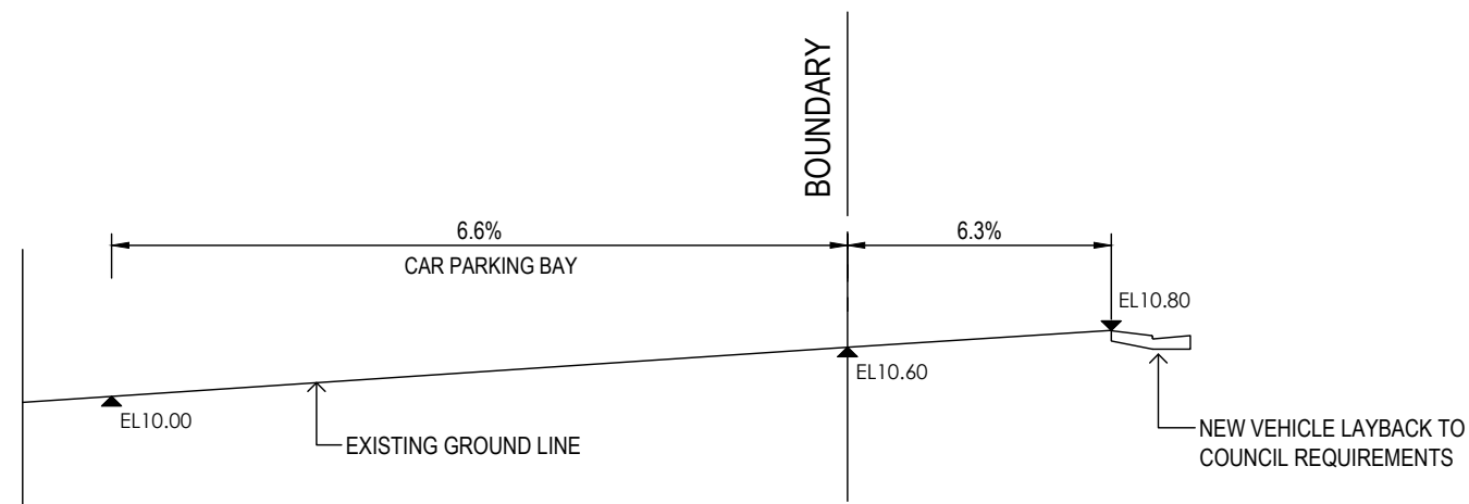
DRIVEWAY LONG SECTION SECTION A-A
