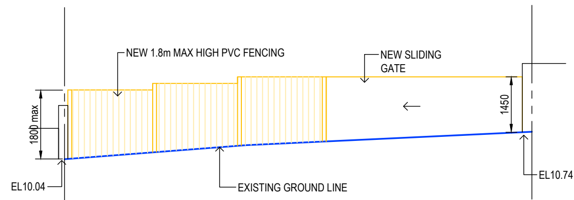
ELEVATION AT FRONT FENCE
