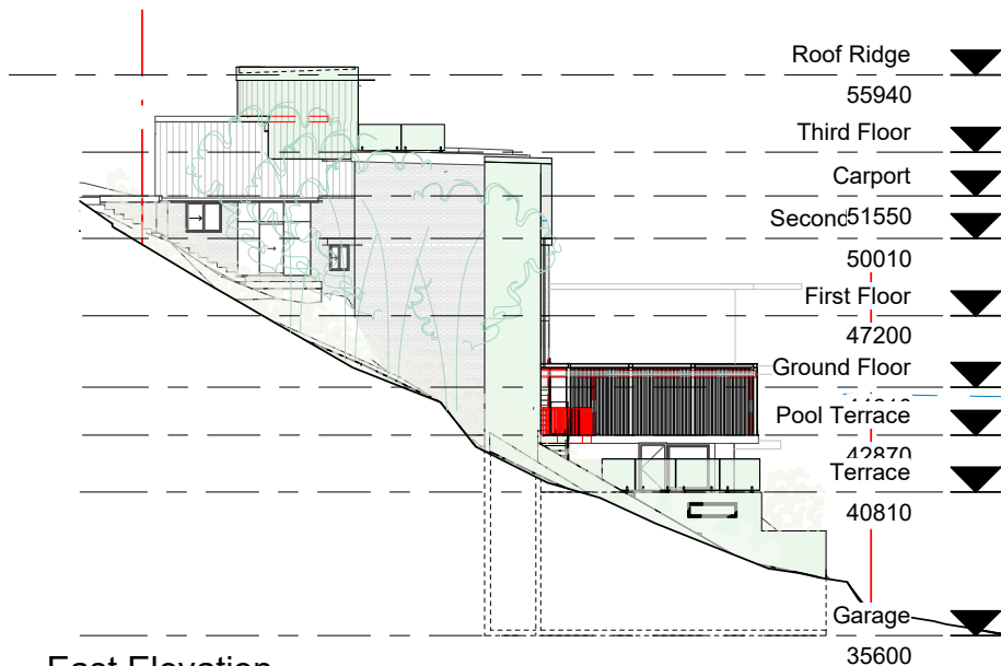
2 East Elevation 1 : 300
