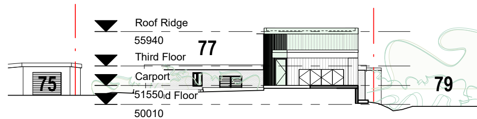
4 South Elevation 1 : 300
