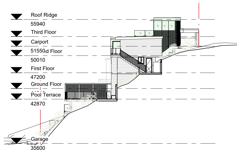
5 West Elevation 1 : 300
