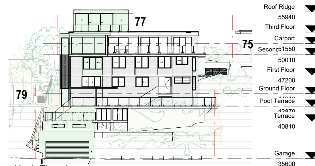
3 North Elevation 1 : 300
