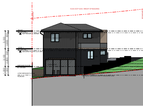
4 NORTH ELEVATION 1:400
