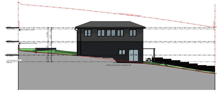
3 EAST ELEVATION 1:400
