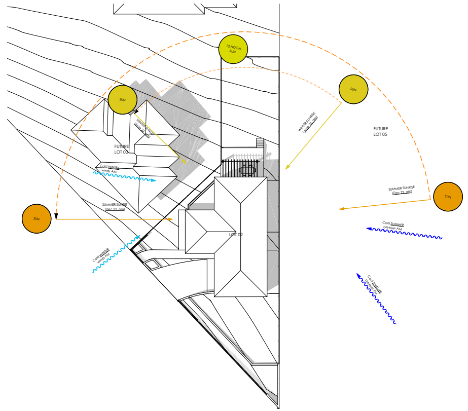
5 SITE ANALYSIS PLAN 1:500
