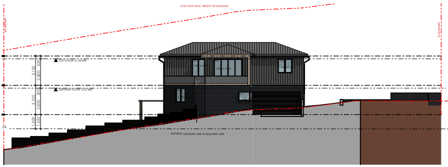
1 WEST ELEVATION 1:400
