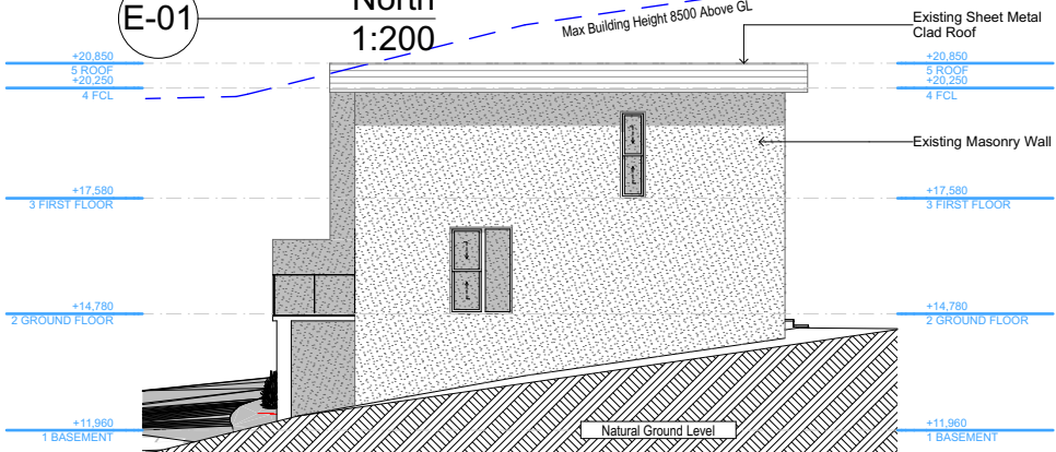
E-02 East 1:200
