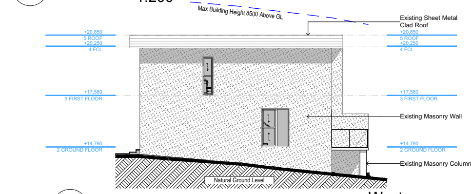
E-04 West 1:200
