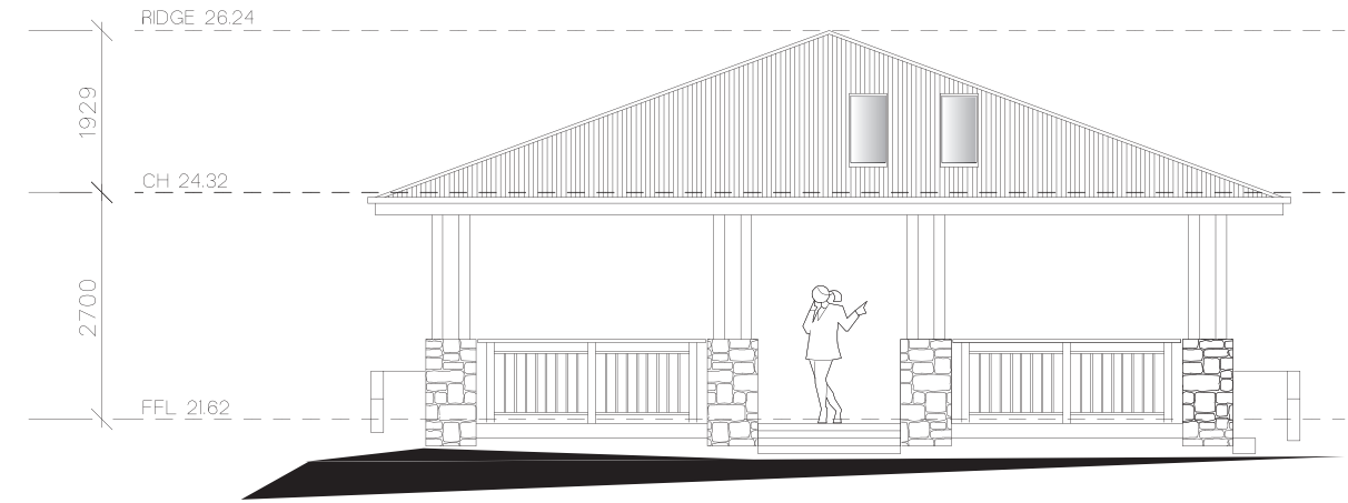
NORTH EAST ELEVATION 1 : 100
