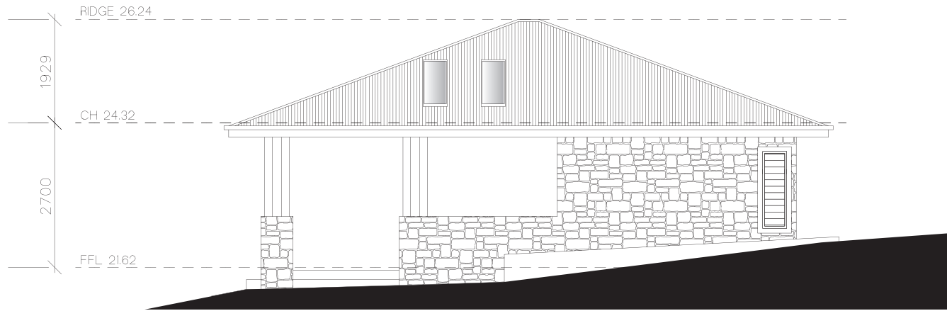
NORTH WEST ELEVATION 1 : 100
