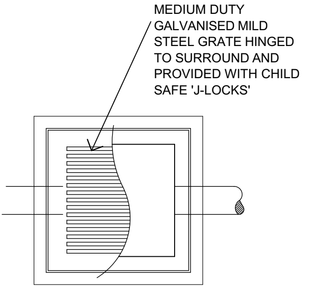
PLAN SECTION STORMWATER PIT DETAIL NOT TO SCALE
