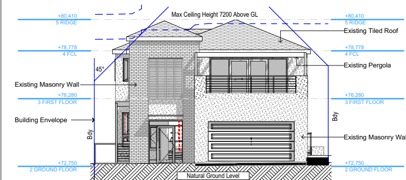
West 1:200
