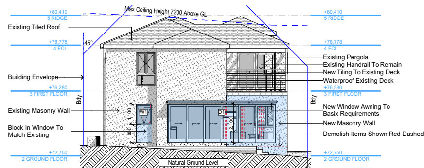
East 1:200
