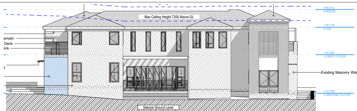
North 1:200
