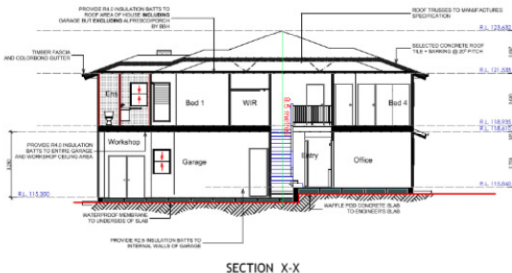
Image 1 - Building Height Calculation
