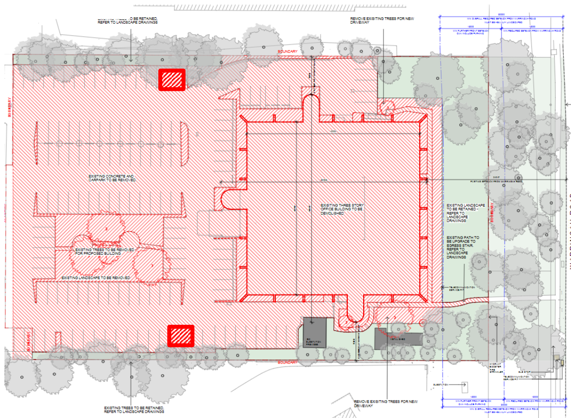
Excerpt – WMK, Drawing DA020, Issue 3, dated 17.09.2021 – Demolition Plan
