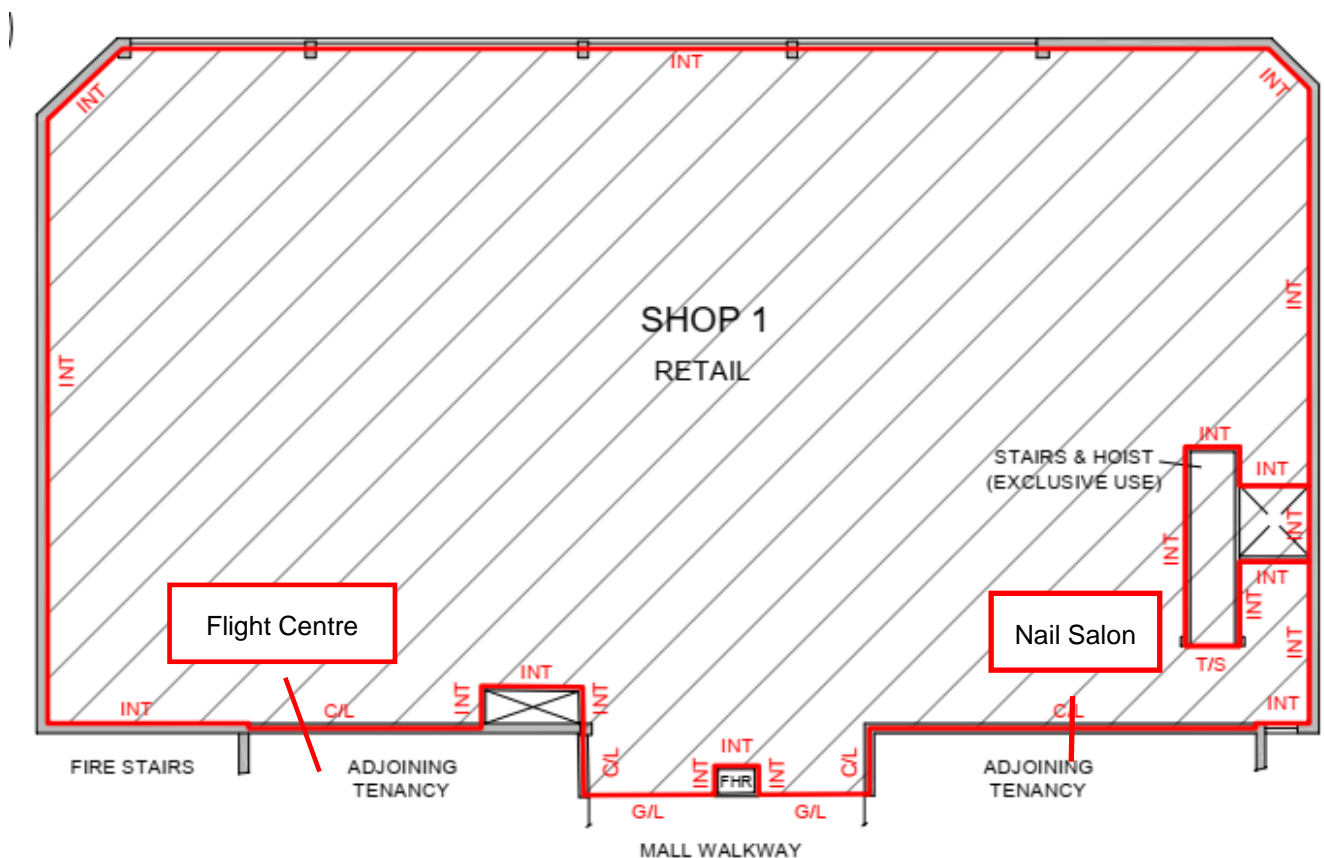
Figure 2-1 Shop Layout
