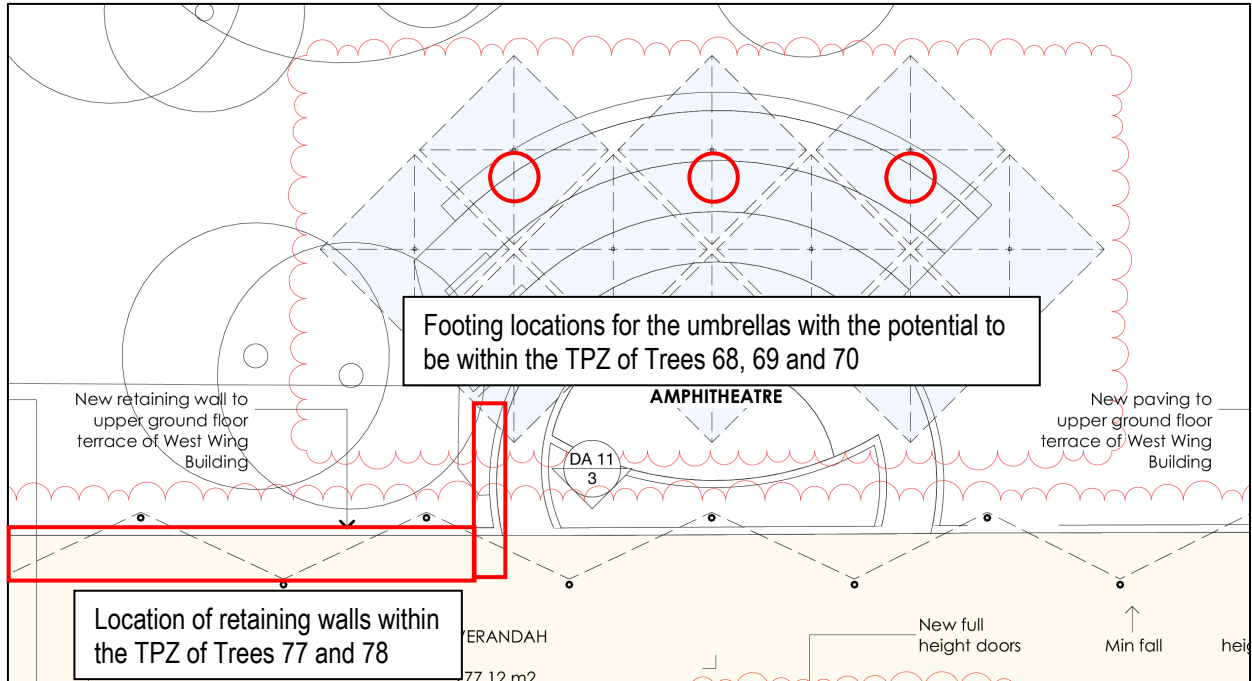
Figure 7. Site map showing tree requiring specific protection measures (Plan No. 6692). (Neeson Murcutt Architects, 19 May 2021).
