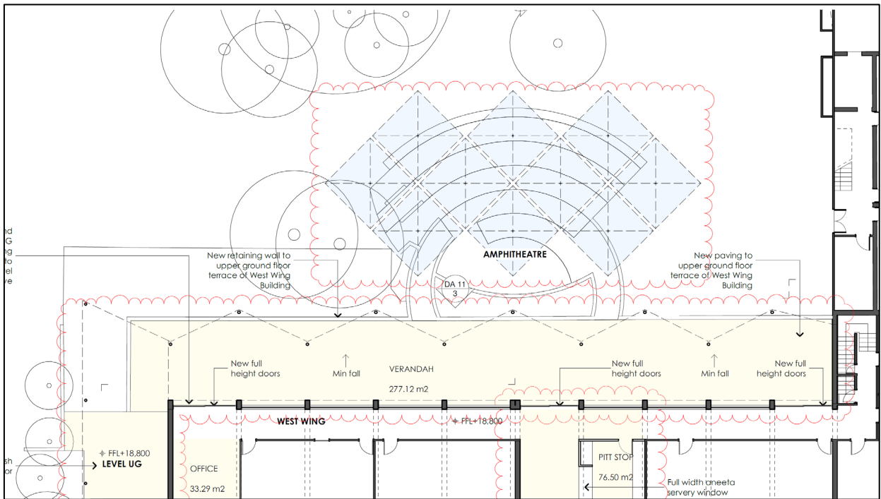
Figure 2. Excerpt from The Pittwater House Schools GA – First Floor (Plan No. 6692). (Neeson Murcutt Architects Pty Ltd, 19 May 2021).
