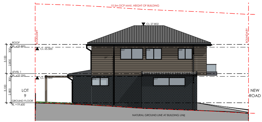
2 EAST ELEVATION 1:250
