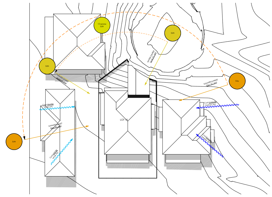
5 SITE ANALYSIS PLAN 1:500
