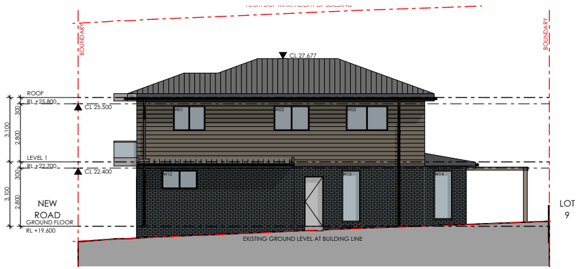
1 WEST ELEVATION 1:250
