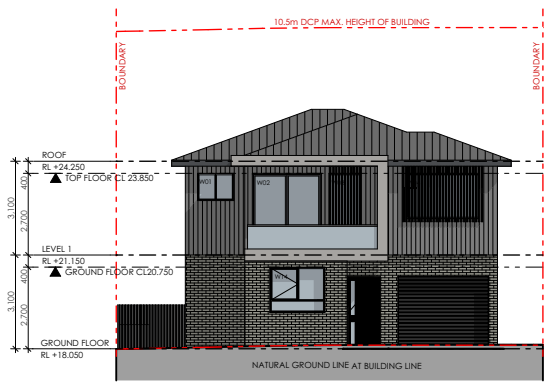
1 WEST ELEVATION 1:250
