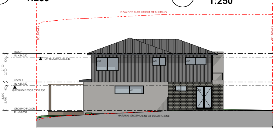
3 NORTH ELEVATION 1:250
