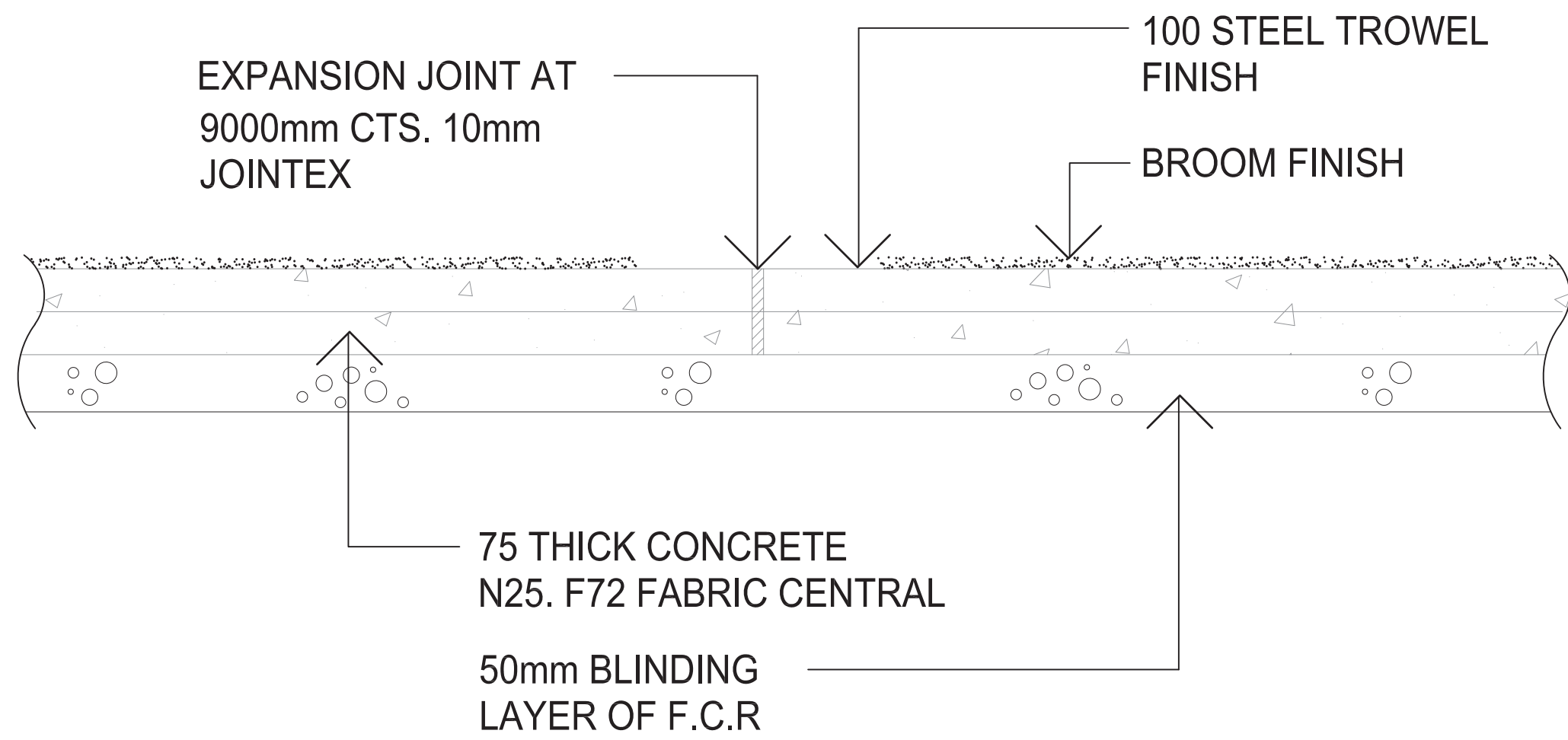
SECTION 1:10 - EXPANSION JOINT
