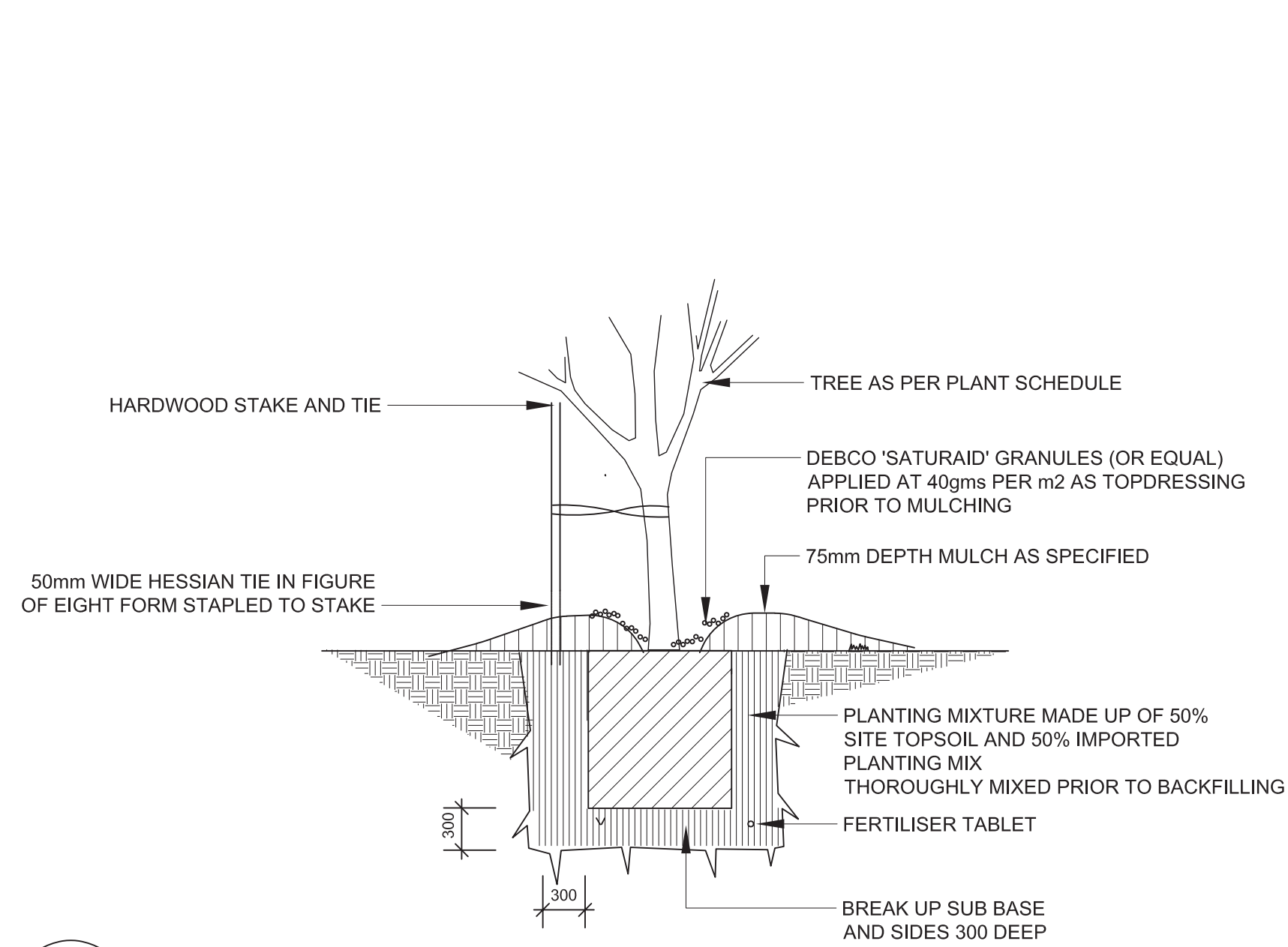
1 TREE PLANTING (75L) TYPICAL SECTION 1:20 NOTE: ENSURE PLANTS ARE WATERED THOROUGHLY PRIOR TO PLANTING AND IMMEDIATELY FOLLOWING PLANTING INSTALLATION
