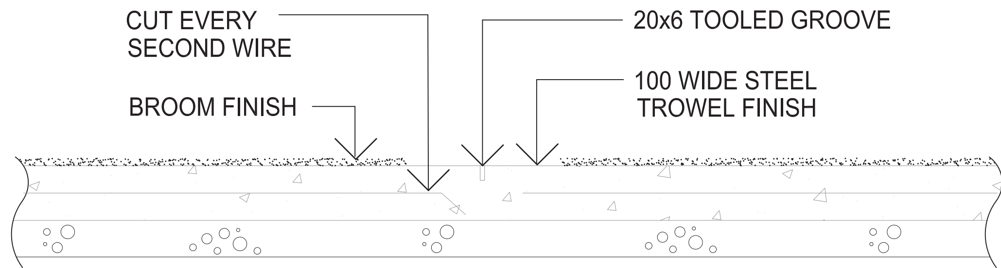
SECTION 1:10 - CONSTRUCTION JOINT
