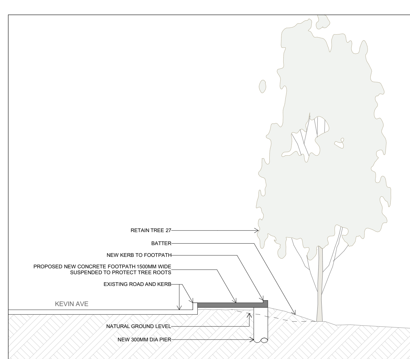
SECTION A - PROPOSED PATHWAY 1:50
