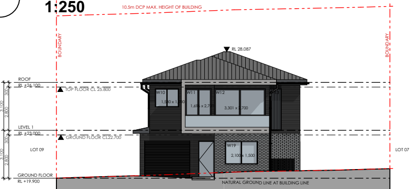
4 SOUTH ELEVATION 1:250
