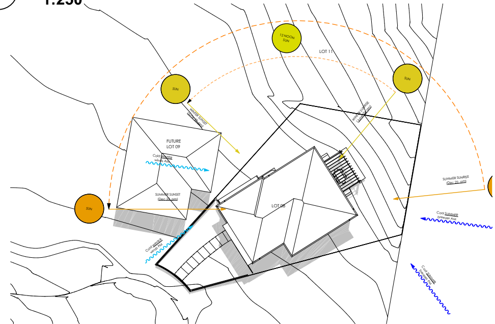
5 SITE ANALYSIS PLAN 1:500
