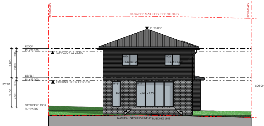
3 NORTH ELEVATION 1:250
