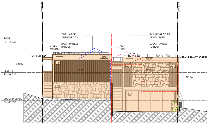
1 NORTH ELEVATION GARAGE 1:200
