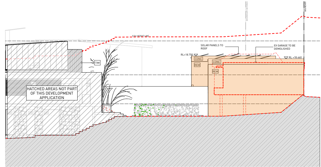
4 WEST ELEVATION 1:200
