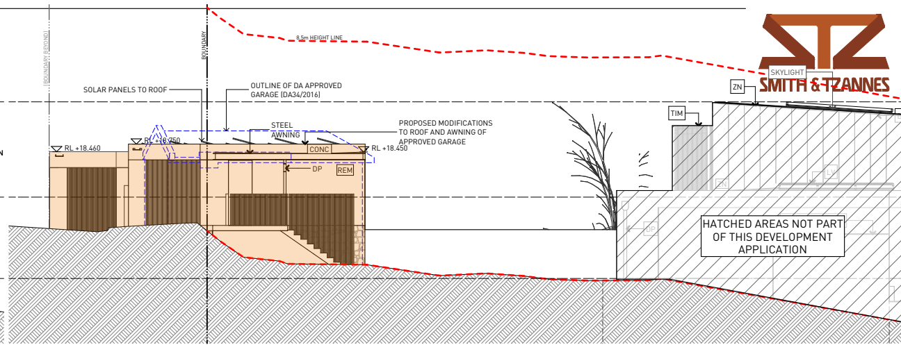
2 EAST ELEVATION 1:200
