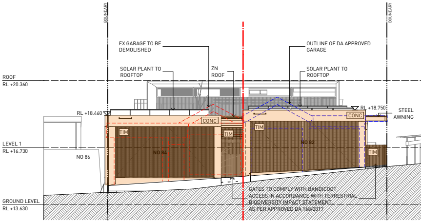
3 SOUTH ELEVATION GARAGE 1:200
