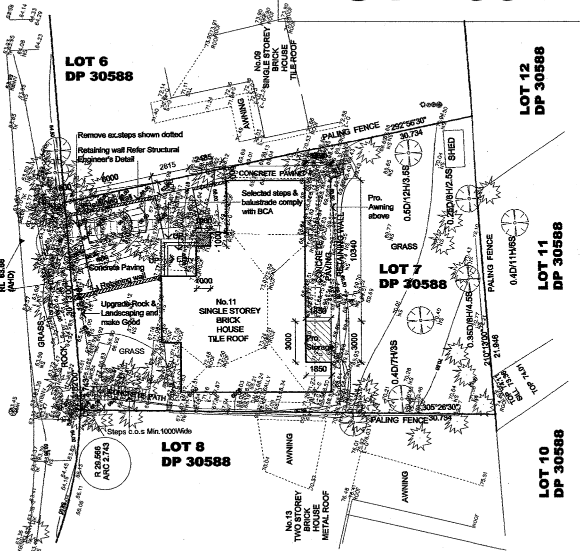
01 Proposed Site Plan C.O.S - CONFIRM ON SITE 1:200@A3
