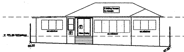
01 Proposed North Elevation C.O.S - CONFIRM ON SITE 1:100@A3
