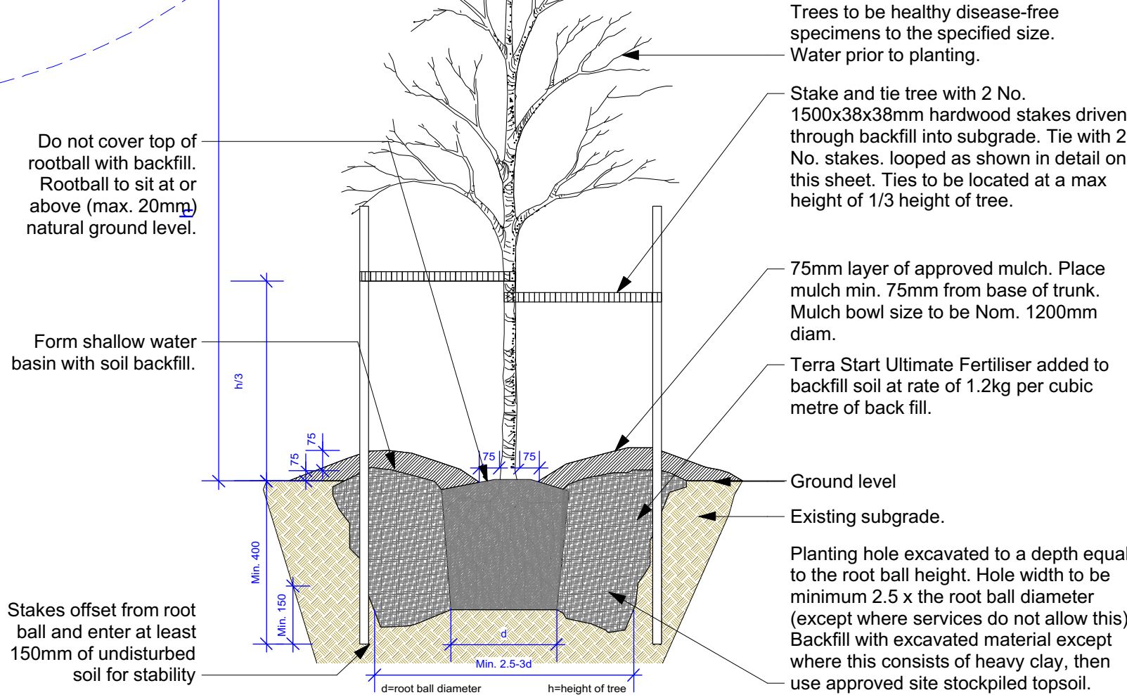
2 Tree planting Scale: 1:20
