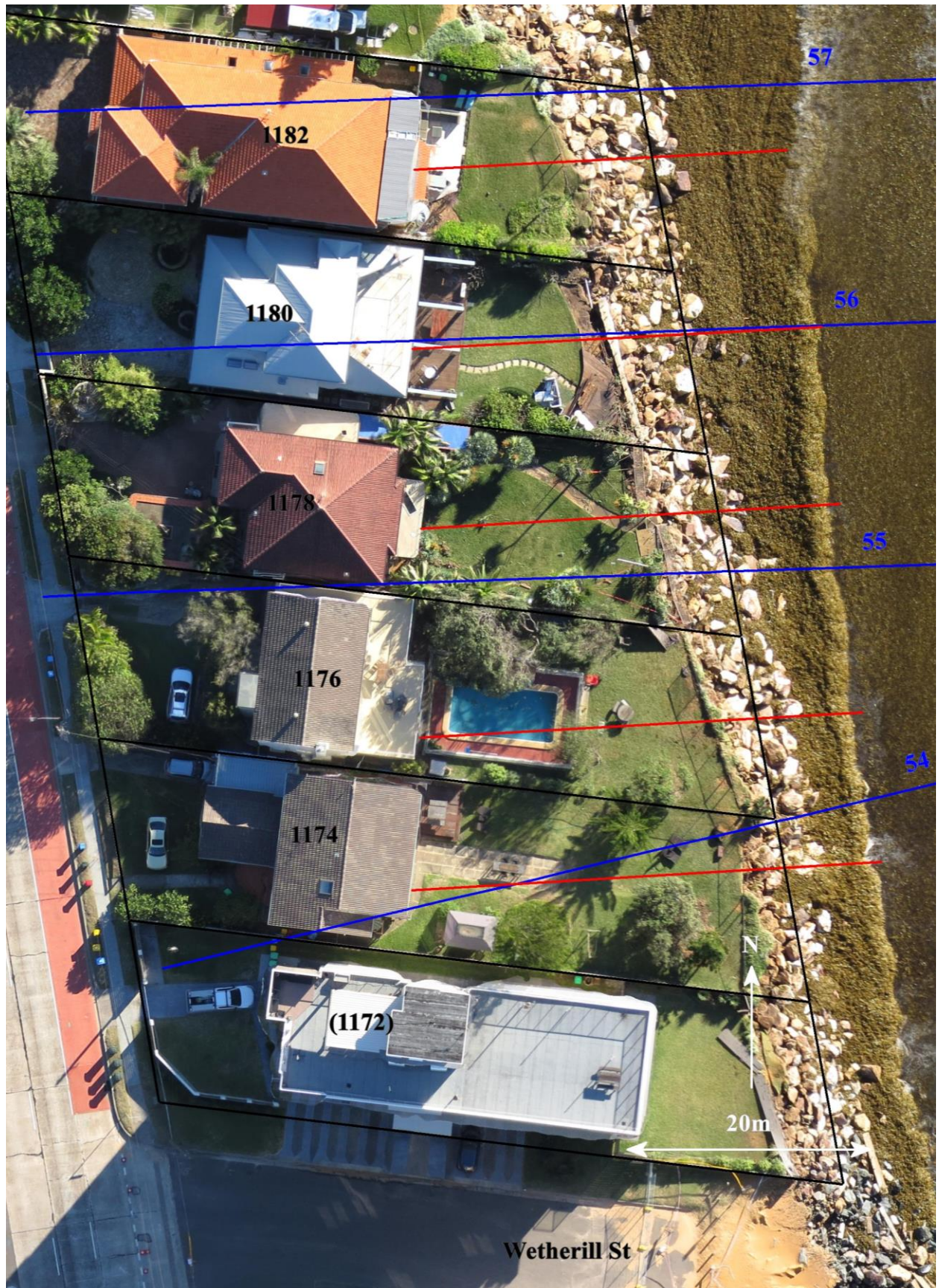
Figure 23: Location of cross sections at each property (red) and OEH profiles (blue), overlaid on 10 June 2016 aerial photograph
