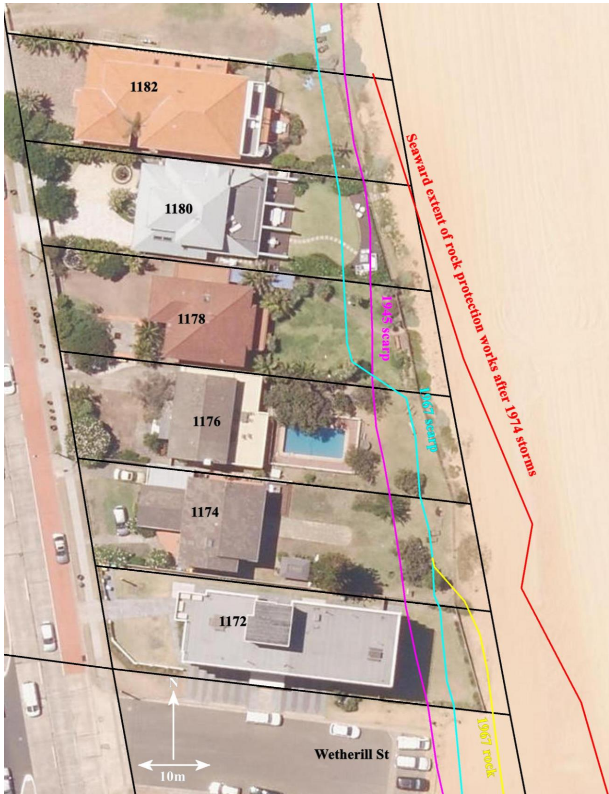
Figure 5: Erosion escarpment at subject properties after 1945 and 1967 storm, and extent of 1967 and 1974 rock protection works, overlaid on 4 January 2014 aerial photograph
