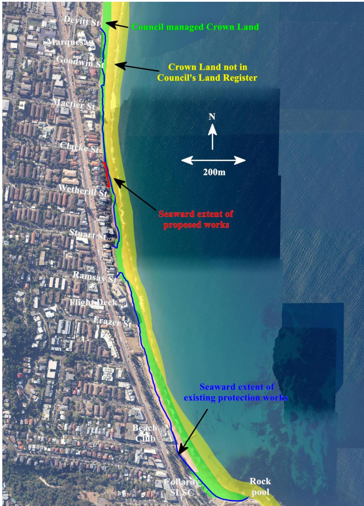
Figure 3: Extent of proposed (red) and existing (blue) coastal protection works at Collaroy-Narrabeen Beach in relation to Council managed Crown Reserve (green) and Crown Land not in Council's Land Register (yellow)
