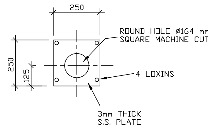
ORIFICE PLATE 1:10
