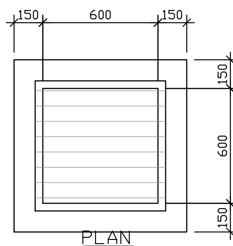
TYPICAL TRANSITION PIT DETAIL 1:20
