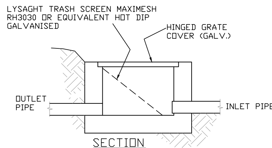
TYPICAL TRANSITION PIT DETAIL 1:20
