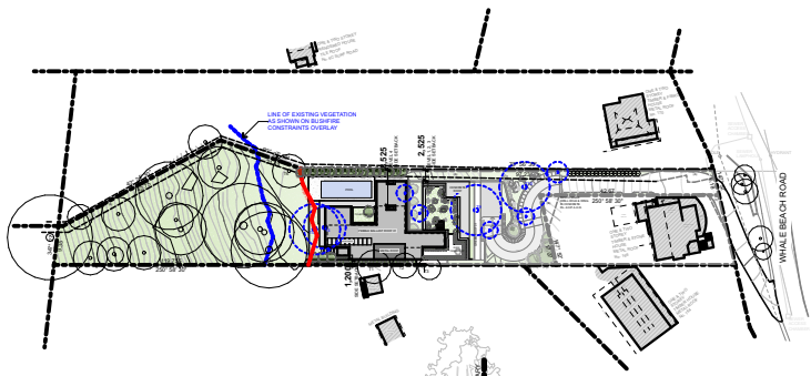
SITE PLAN
