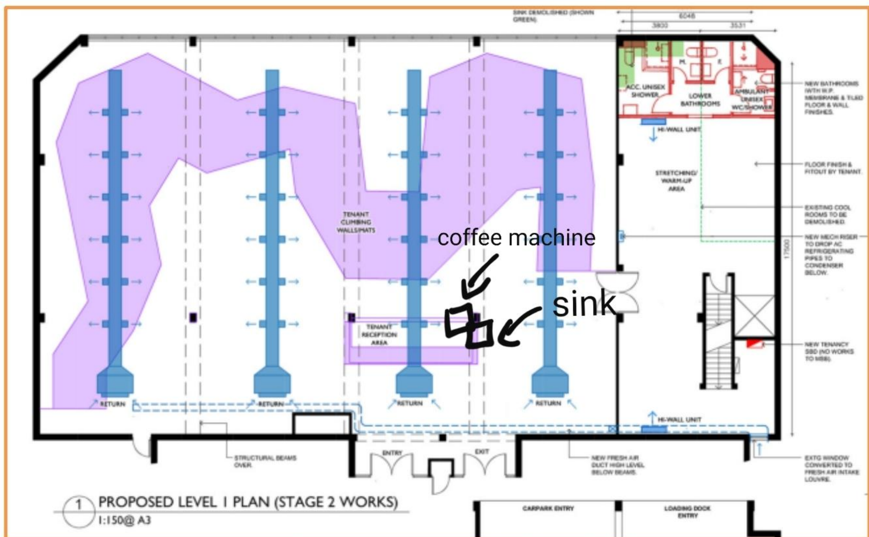
Figure 7: Proposed ground floor plan
