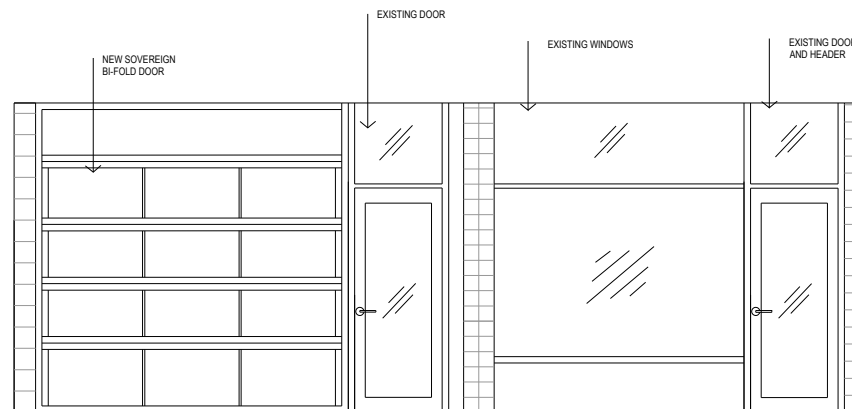
ELEVATION F
