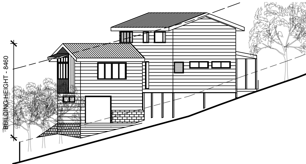
SOUTH-EAST ELEVATION
