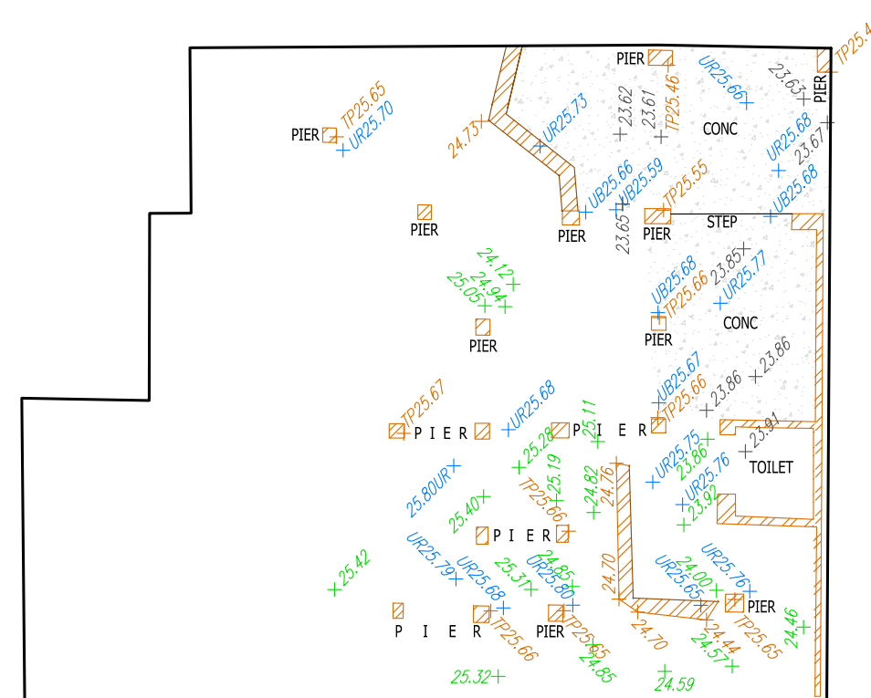
BASEMENT INTERNAL PLAN
