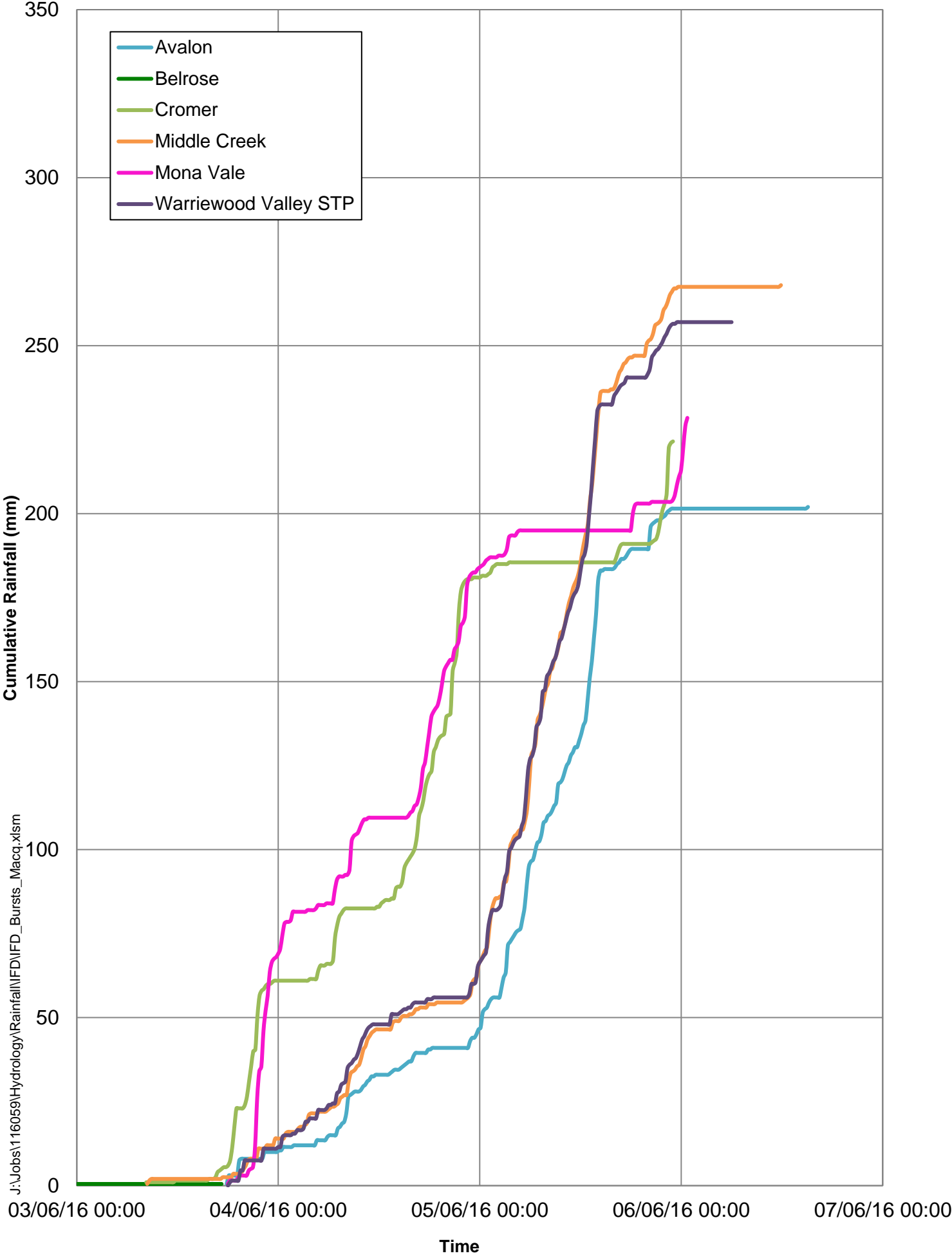
FIGURE 8E RECORDED CUMULATIVE RAINFALL DEPTHS JUNE 2016 RAINFALL EVENT
