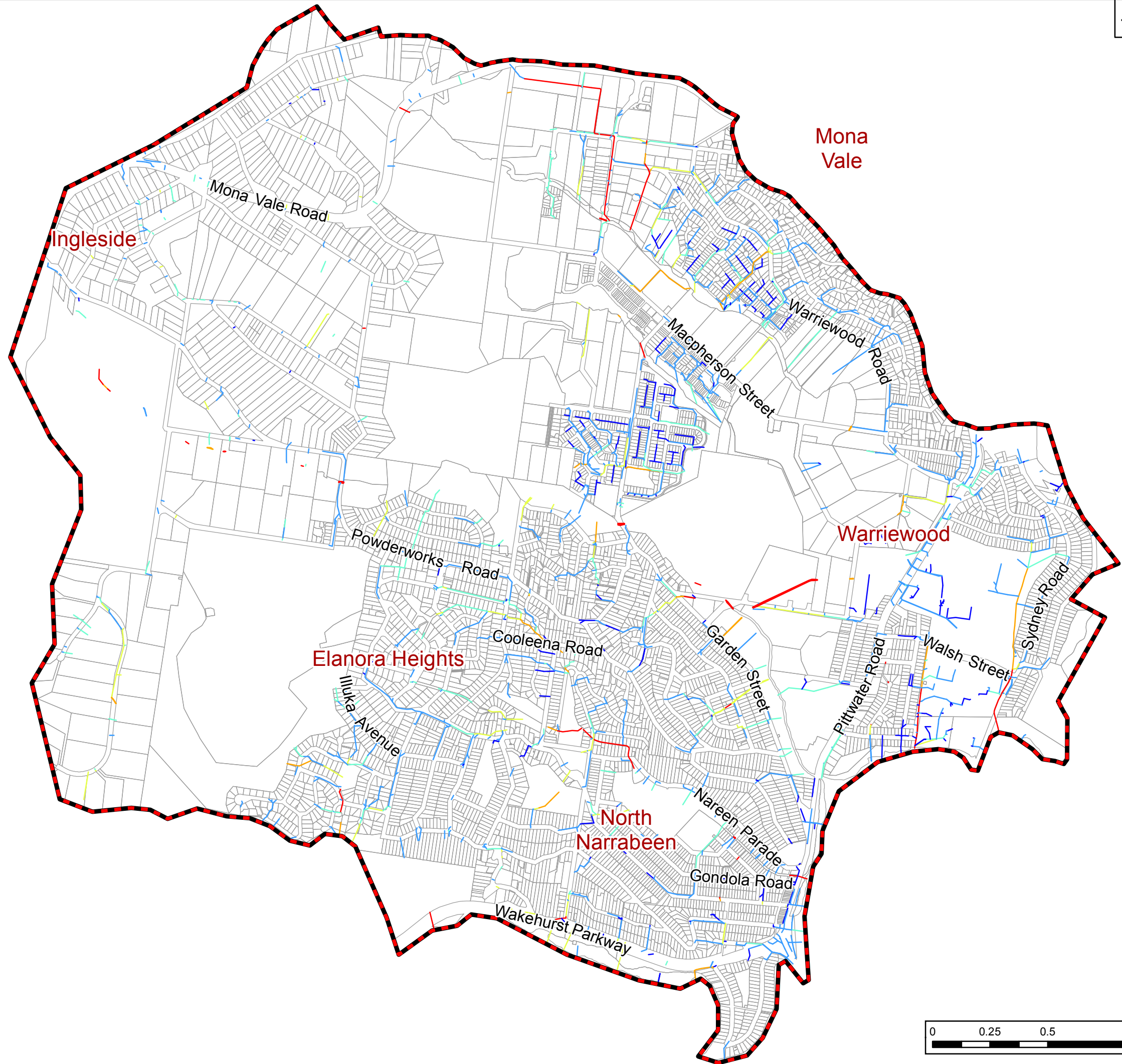
FIGURE 12 TUFLOW PITS AND PIPES
