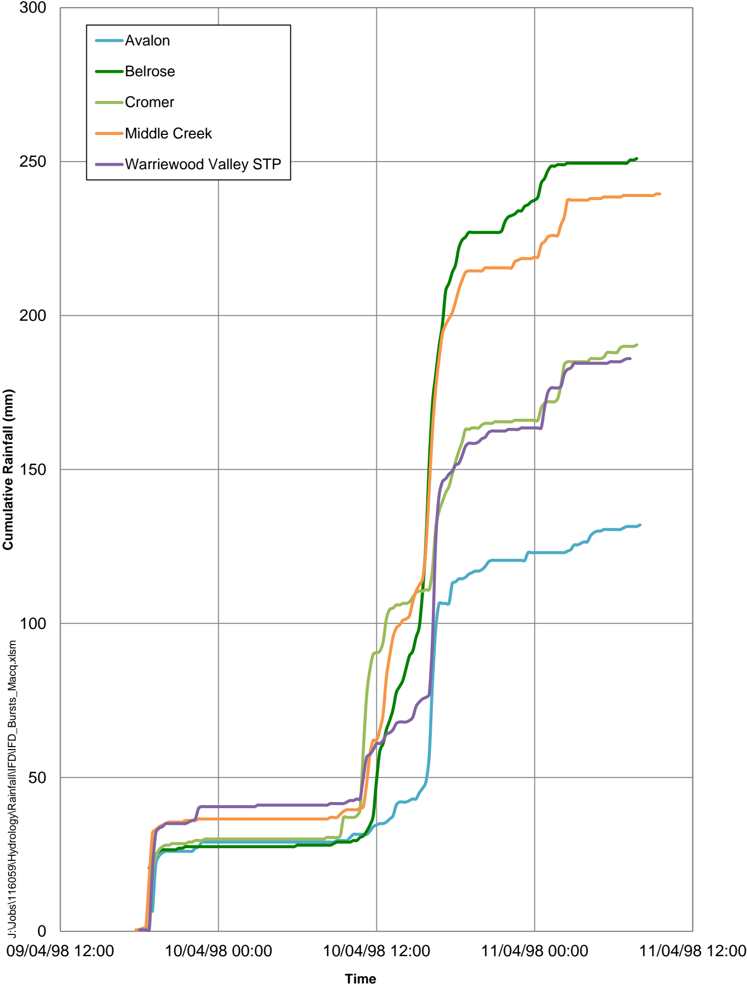
FIGURE 8A RECORDED CUMULATIVE RAINFALL DEPTHS APRIL 1998 RAINFALL EVENT
