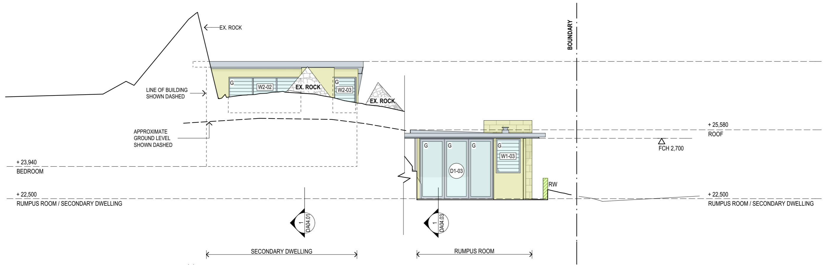
1 WEST ELEVATION 1:100
