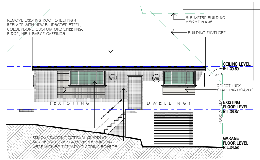
EAST ELEVATION 1:100
