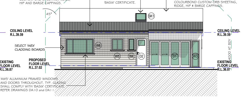
WEST ELEVATION 1:100
