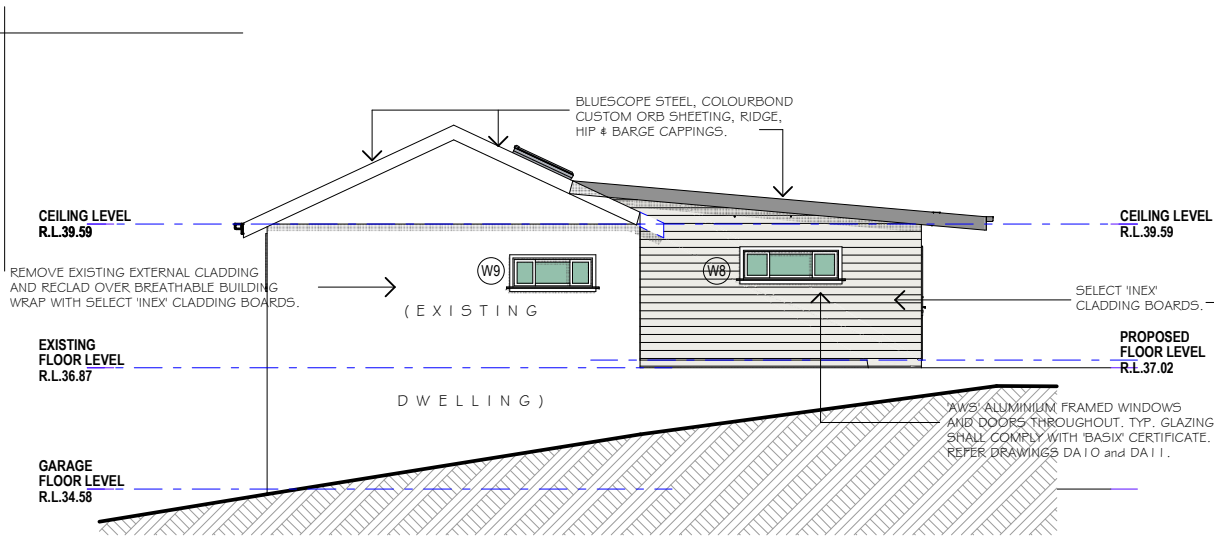
NORTH ELEVATION 1:100
