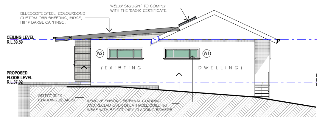
SOUTH ELEVATION 1:100
