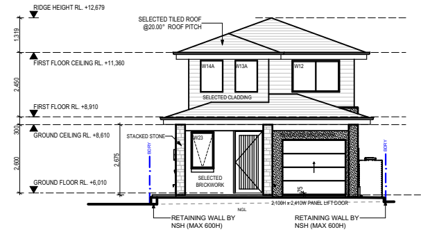
ELEVATION - EAST
