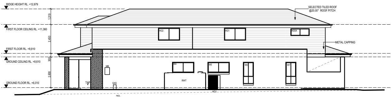
ELEVATION - NORTH
