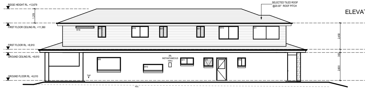
ELEVATION - SOUTH
