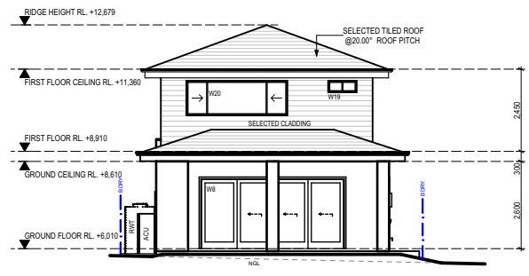
ELEVATION - WEST
