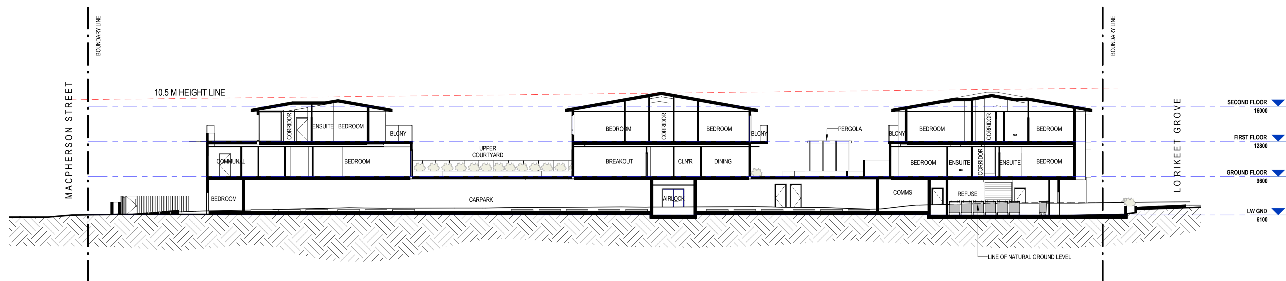
SECTION A
