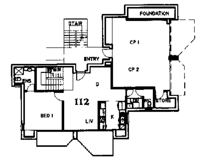
GROUND FLOOR PLAN UNIT CLUSTER - 30
