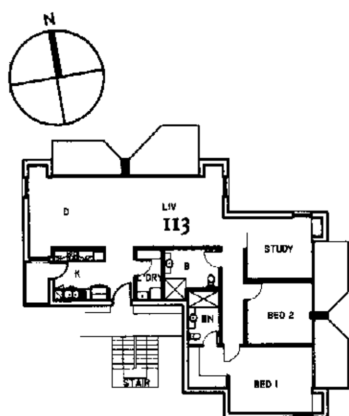
FIRST FLOOR PLAN UNIT CLUSTER - 29
