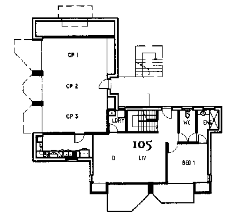
GROUND FLOOR PLAN UNIT CLUSTER - 31
