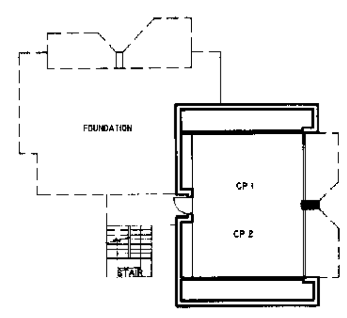
GROUND FLOOR PLAN UNIT CLUSTER - 29
