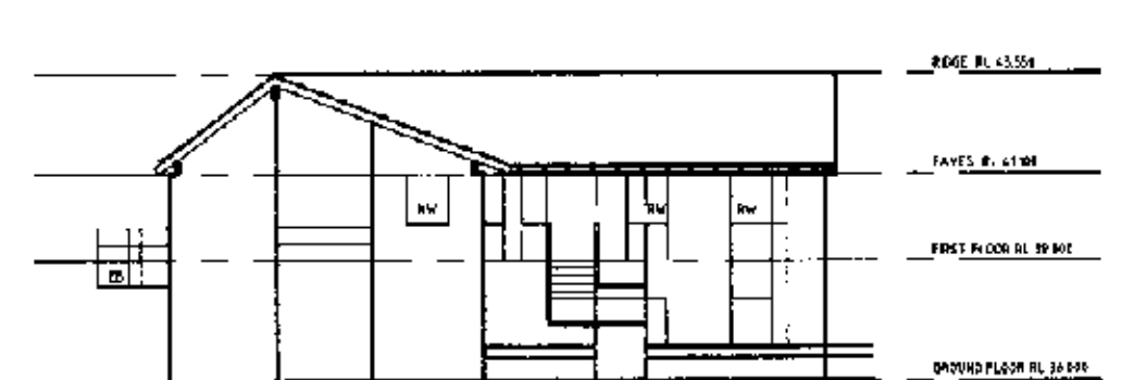
NORTH ELEVATION UNIT CLUSTER - 32
