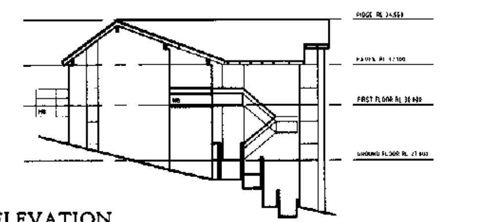
WEST ELEVATION UNIT CLUSTER - 29
