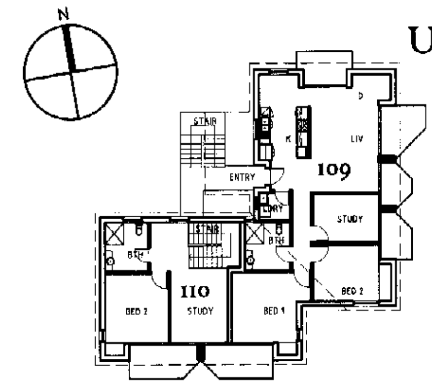
FIRST FLOOR PLAN UNIT CLUSTER - 32
