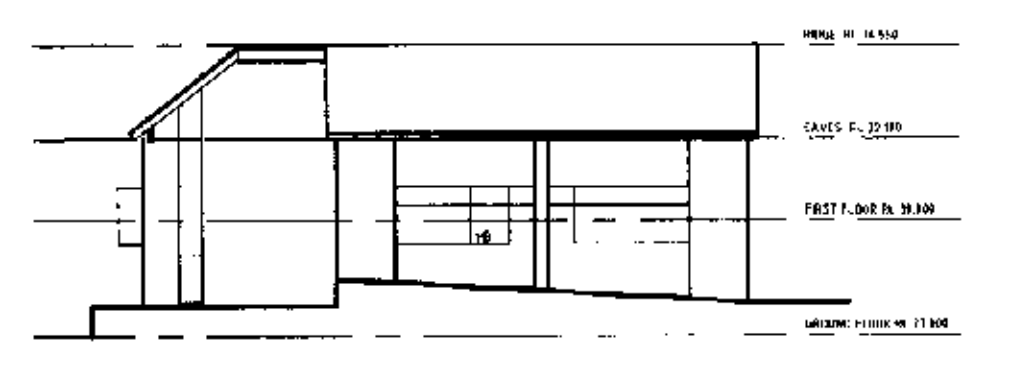
NORTH ELEVATION UNIT CLUSTER - 29
