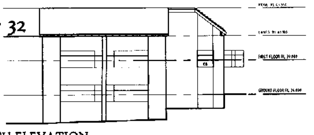
SOUTH ELEVATION UNIT CLUSTER - 32
