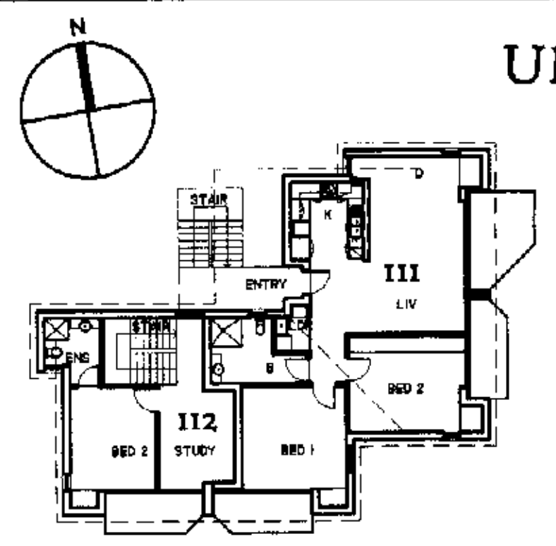
FIRST FLOOR PLAN UNIT CLUSTER - 30
