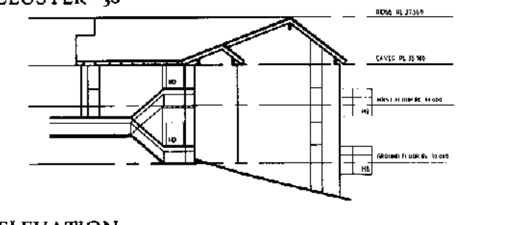
WEST ELEVATION UNIT CLUSTER - 30
