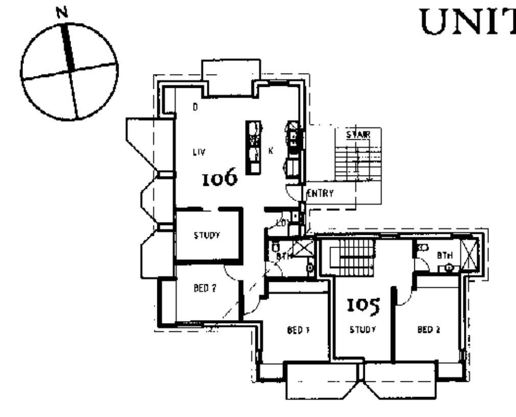
FIRST FLOOR PLAN UNIT CLUSTER - 31
