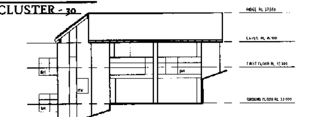
EAST ELEVATION UNIT CLUSTER - 30
