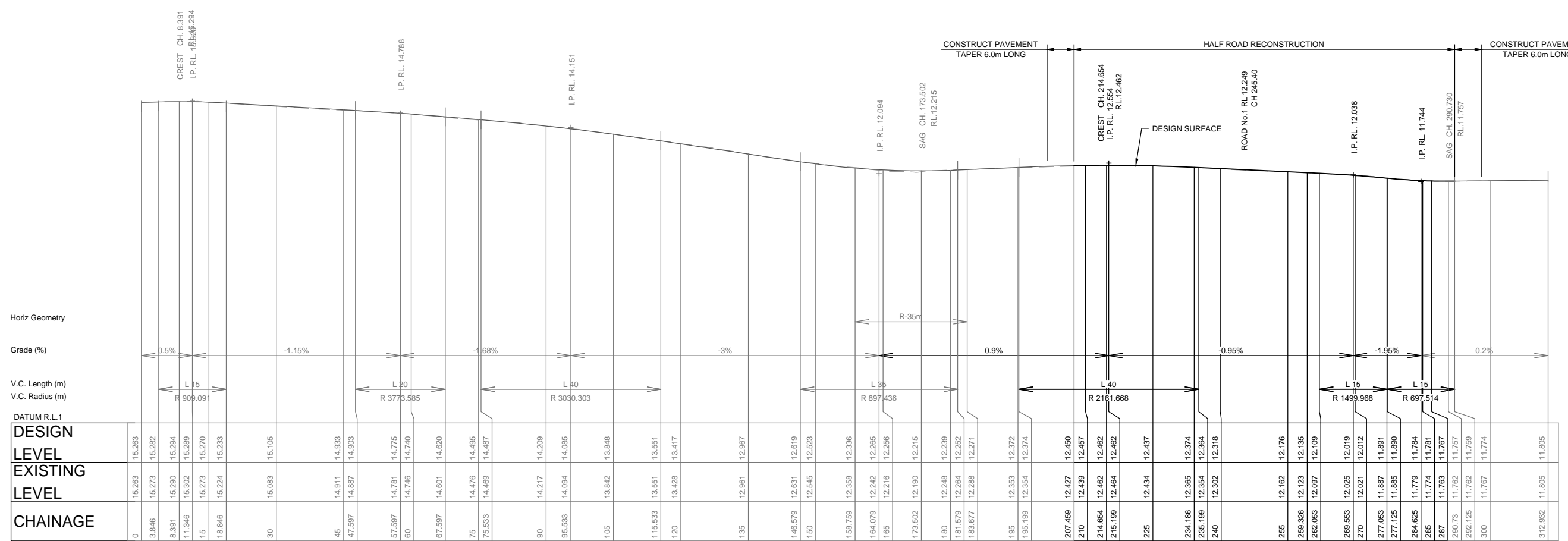
LONGITUDINAL SECTION - WARRIEWOOD RD HORIZONTAL SCALE - 1:500 VERTICAL SCALE - 1:100
