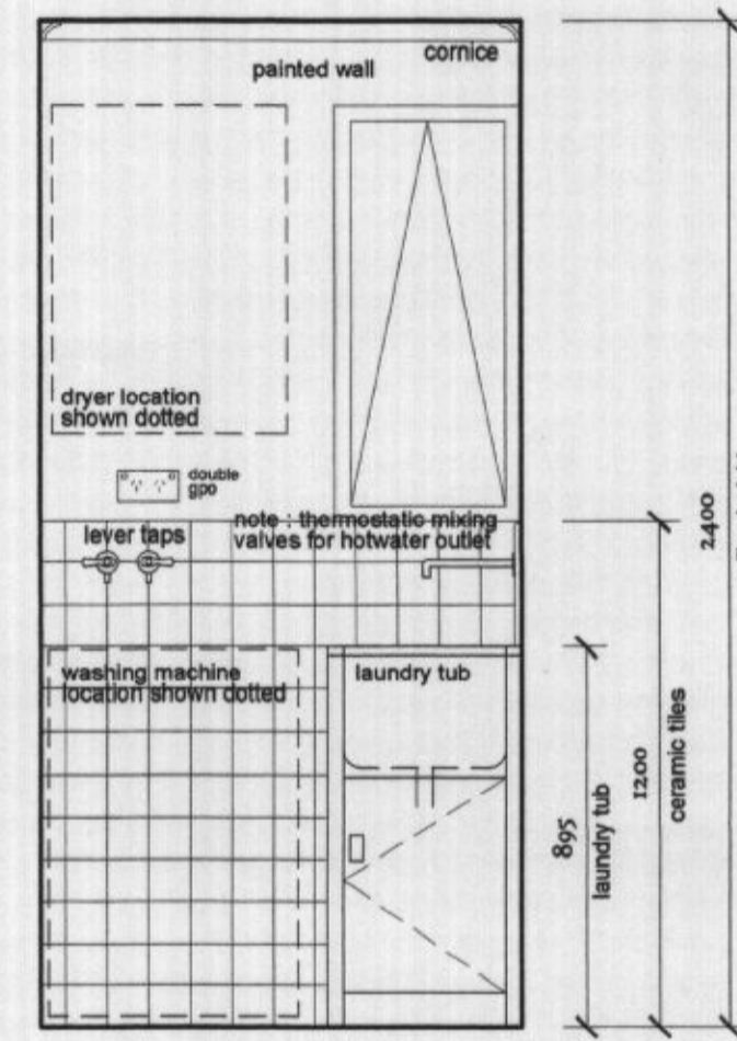
02 LAUNDRY ELEVATION Scale 1:20
