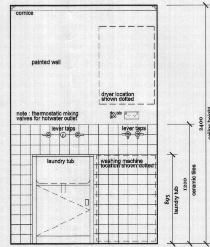
05 LAUNDRY ELEVATION Scale 1:20
