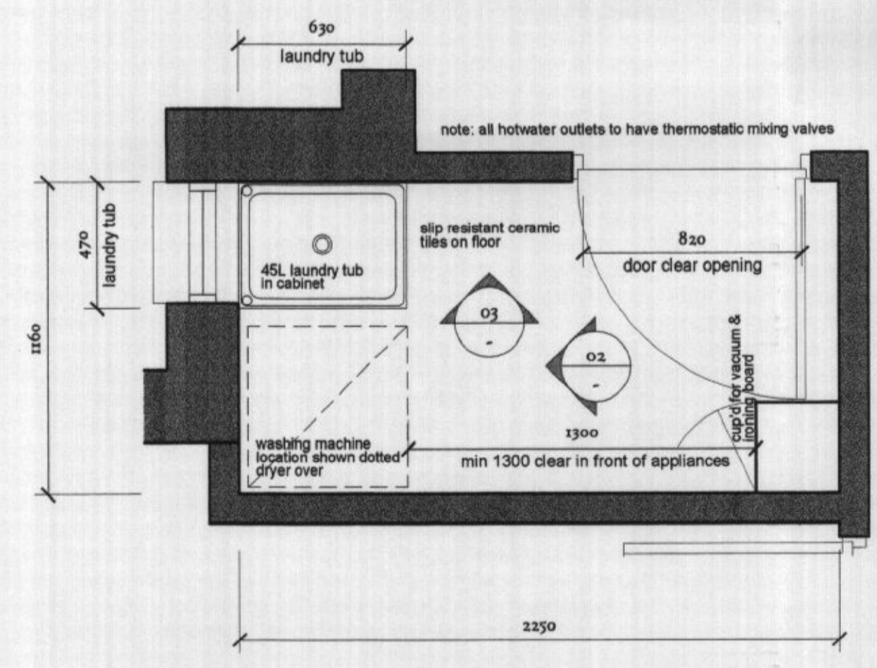
01 LAUNDRY PLAN UNIT 109 Scale 1:20
