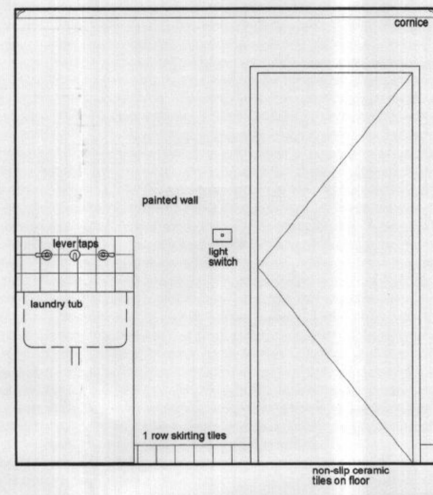
03 LAUNDRY ELEVATION Scale 1:20
