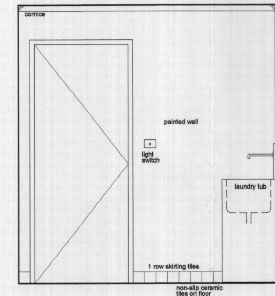
06 LAUNDRY ELEVATION Scale 1:20
