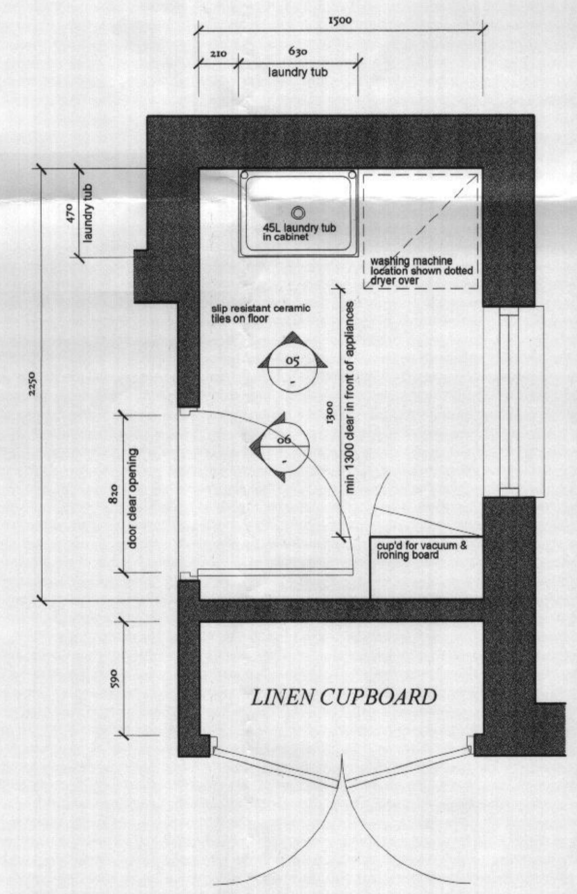
04 LAUNDRY PLAN UNIT 118 Scale 1:20
