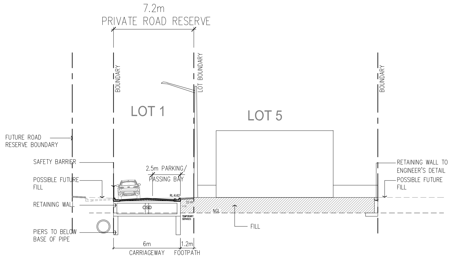
SECTION CC STAGE 1
