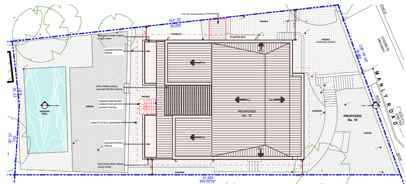
Roof Level 1:400
