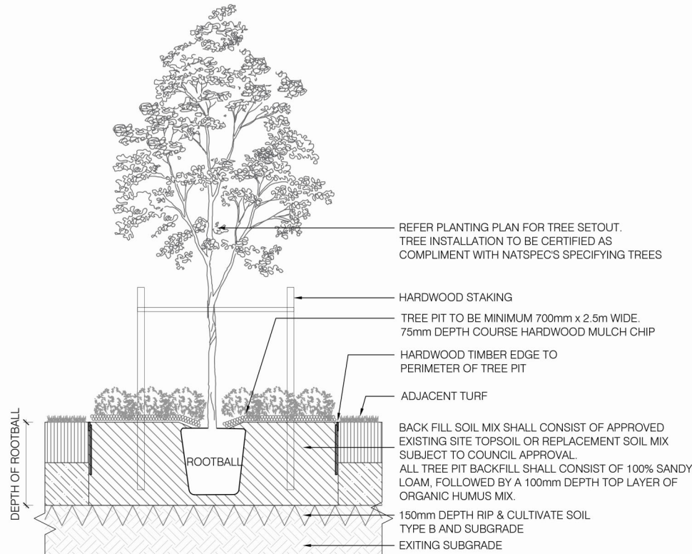
02 TYPICAL TREE IN TURF DETAIL SCALE 1:20 @ A1; 1:40 @ A3
