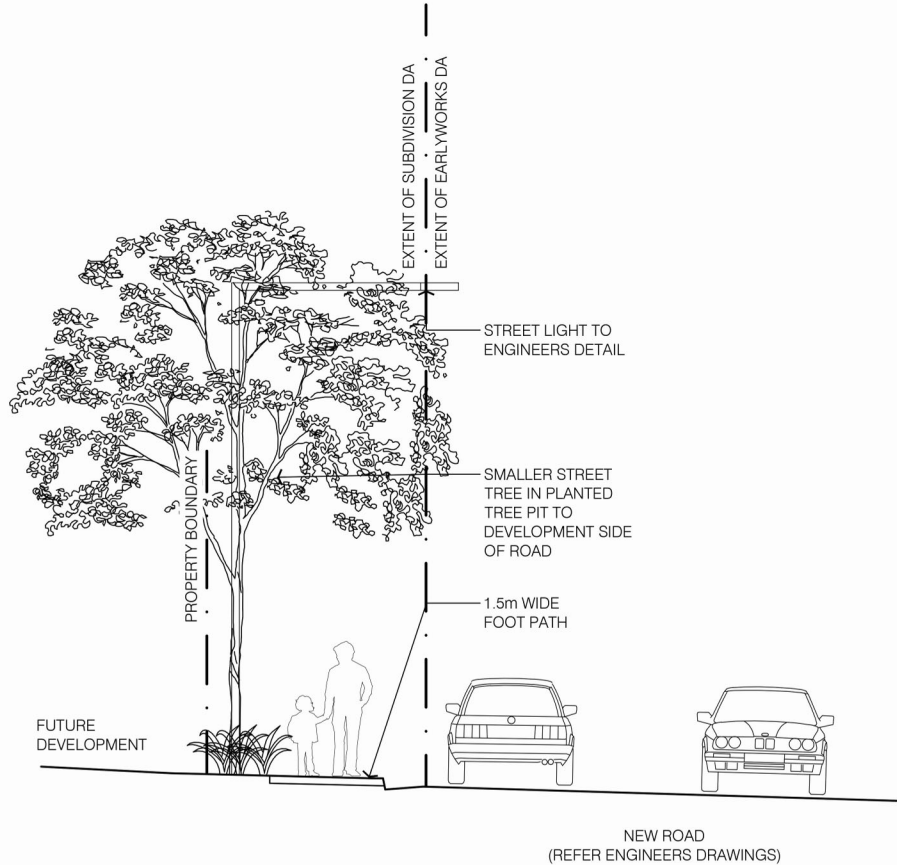
01 TYPICAL LANDSCAPE SECTION SCALE 1:50 @ A1; 1:100 @ A3
