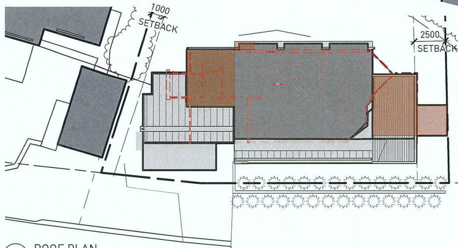
2 ROOF PLAN Scale: 1:300
