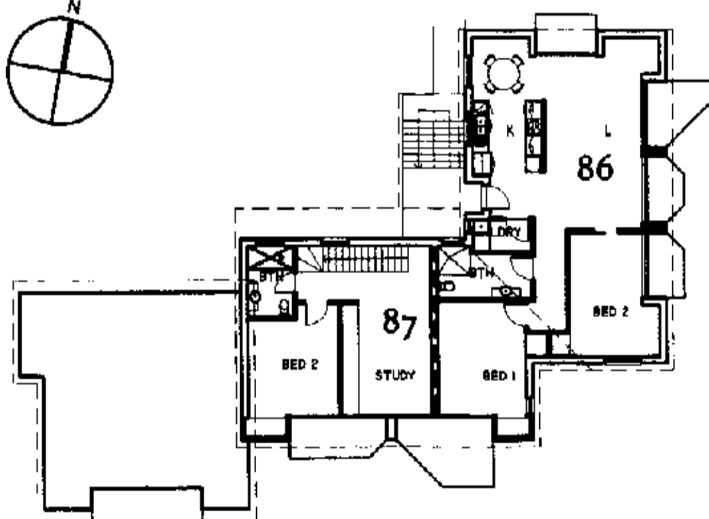
FIRST FLOOR PLAN UNIT CLUSTER - 10
