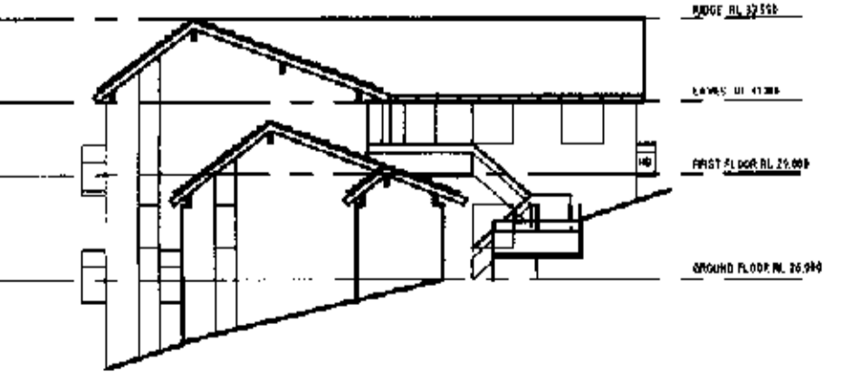
EAST ELEVATION UNIT CLUSTER - 12
