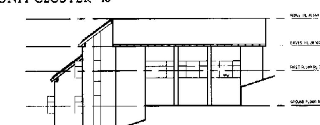
NORTH ELEVATION UNIT CLUSTER - 10
