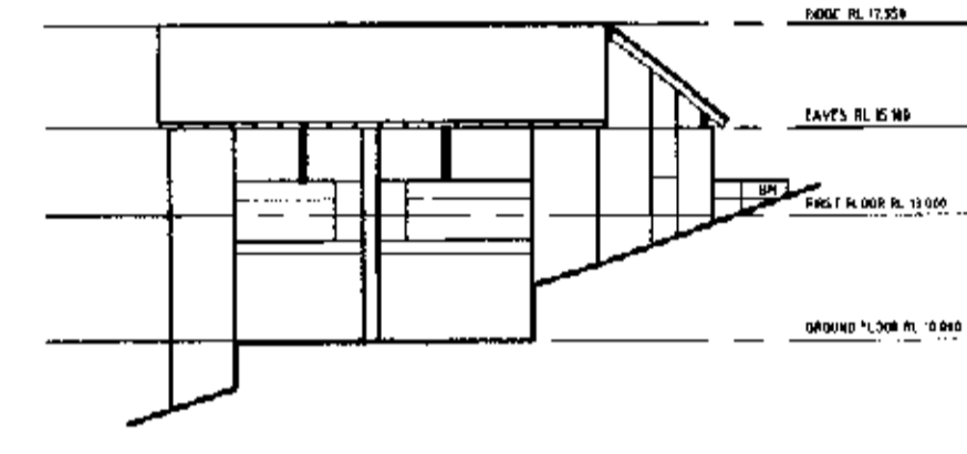
EAST ELEVATION UNIT CLUSTER - 11
