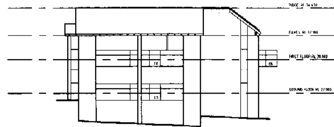
SOUTH ELEVATION UNIT CLUSTER - 09
