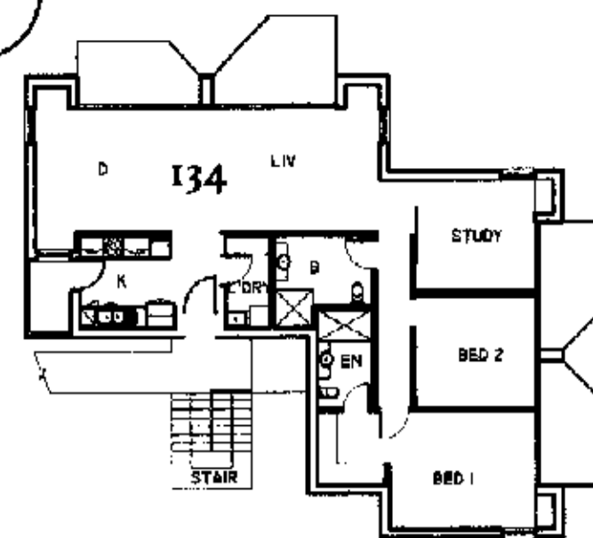
FIRST FLOOR PLAN UNIT CLUSTER - 11
