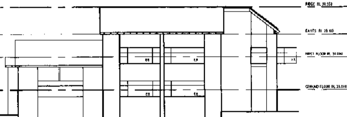
SOUTH ELEVATION UNIT CLUSTER - 10
