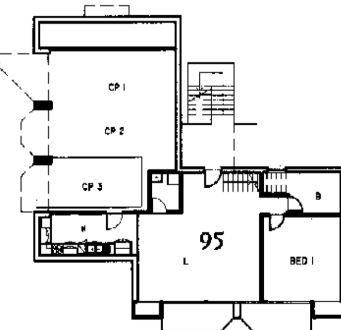
GROUND FLOOR PLAN UNIT CLUSTER - 12
