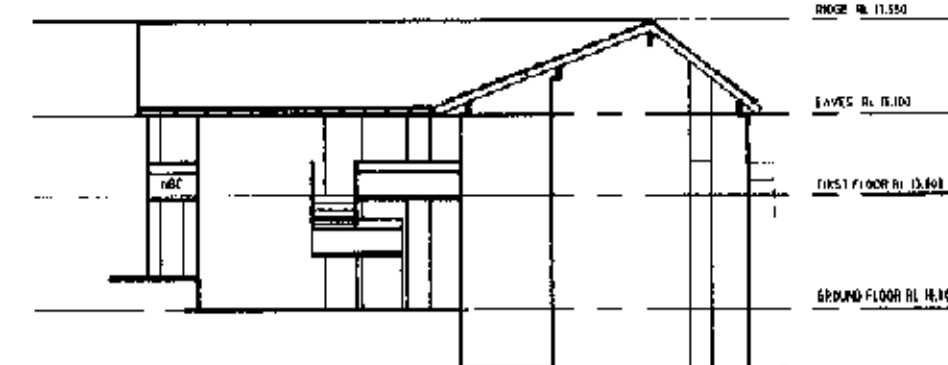
SOUTH ELEVATION UNIT CLUSTER - 11
