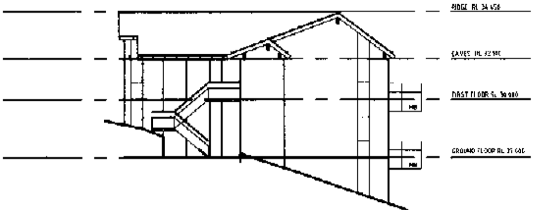
WEST ELEVATION UNIT CLUSTER - 09
