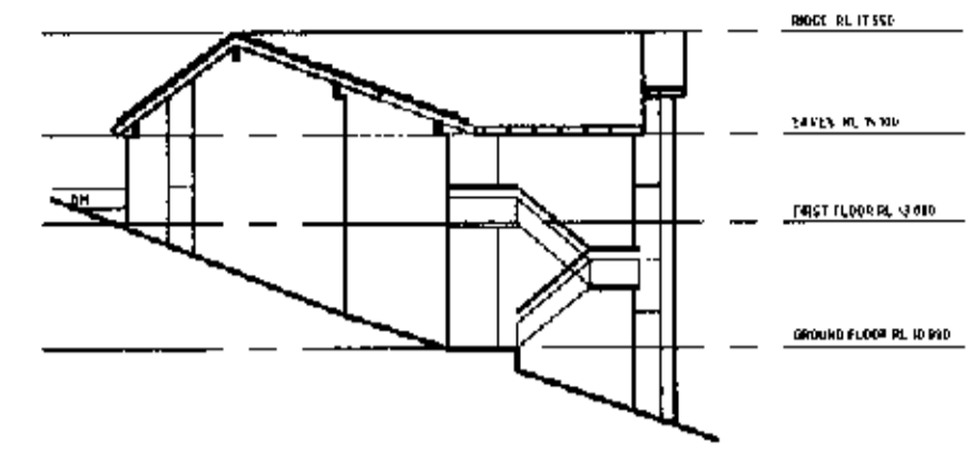
WEST ELEVATION UNIT CLUSTER - 11
