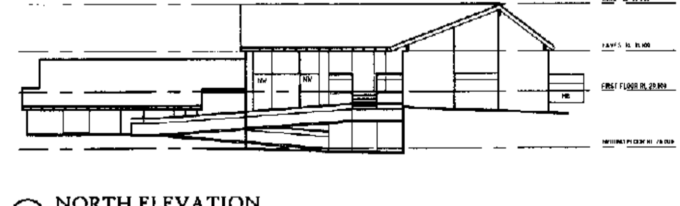
NORTH ELEVATION UNIT CLUSTER - 12
