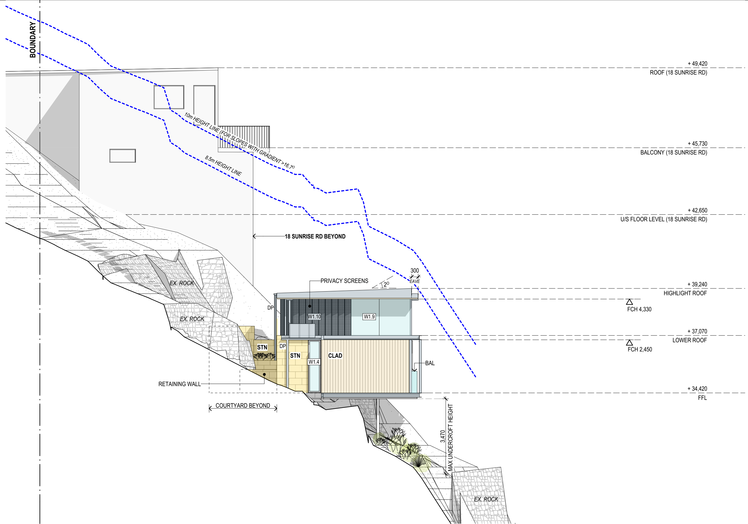
1 SOUTH ELEVATION 1:100
