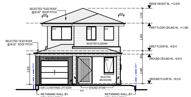
ELEVATION - EAST
