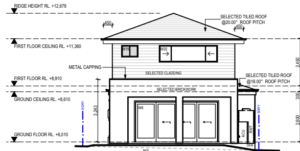
ELEVATION - WEST
