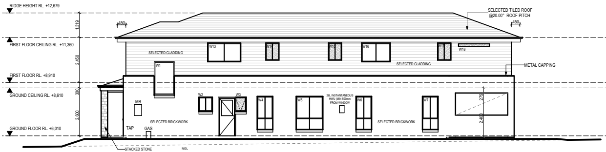
ELEVATION - NORTH
